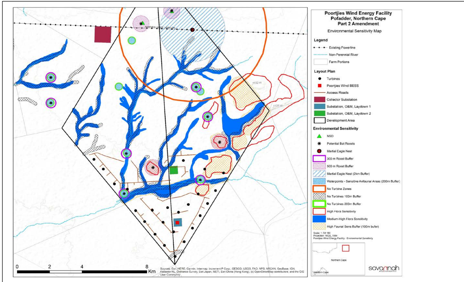
Figure 2.4: Poortjies proposed amendments layout overlain onto the sensitivities (2021) showing turbine positions and associated infrastructures.
