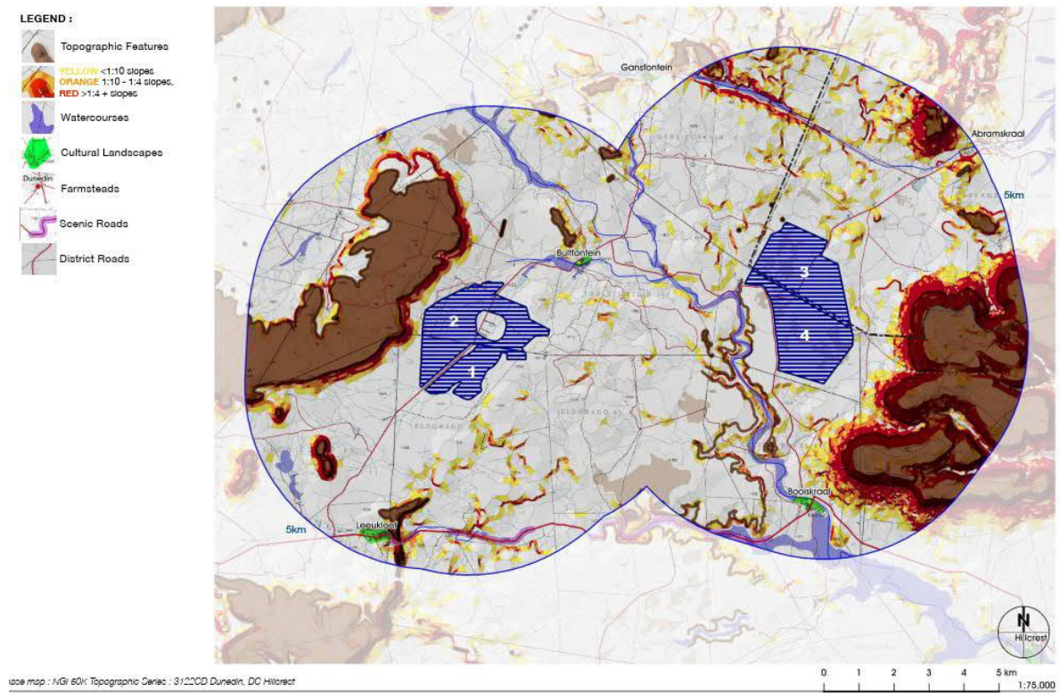
Figure 18: Visual features
