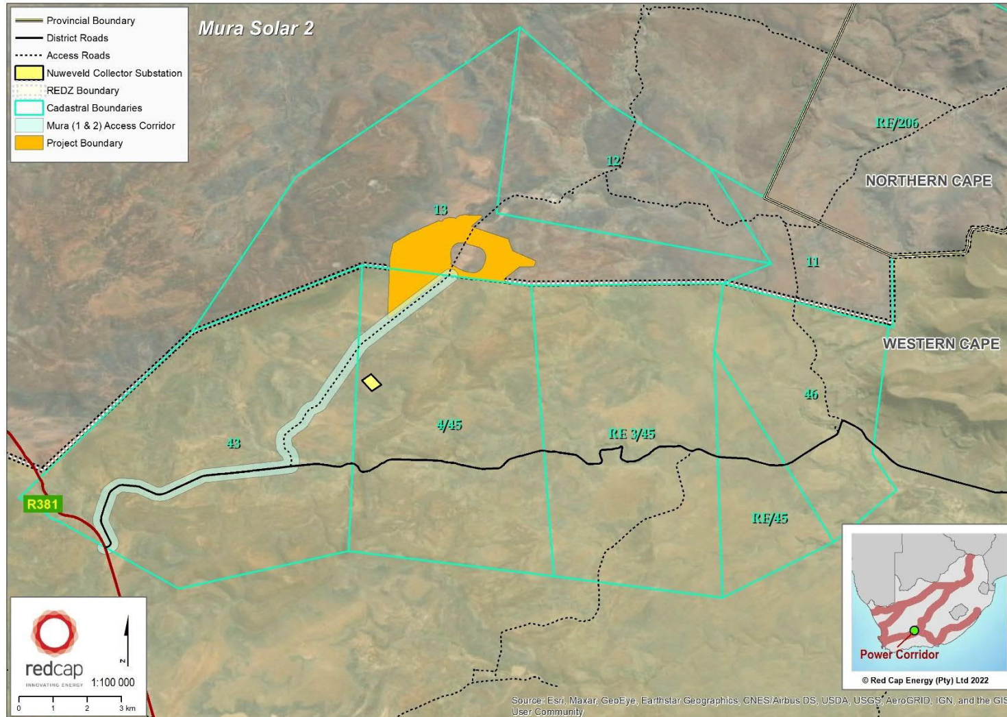
Figure 2-1 – Mura 2 Solar PV Facility
