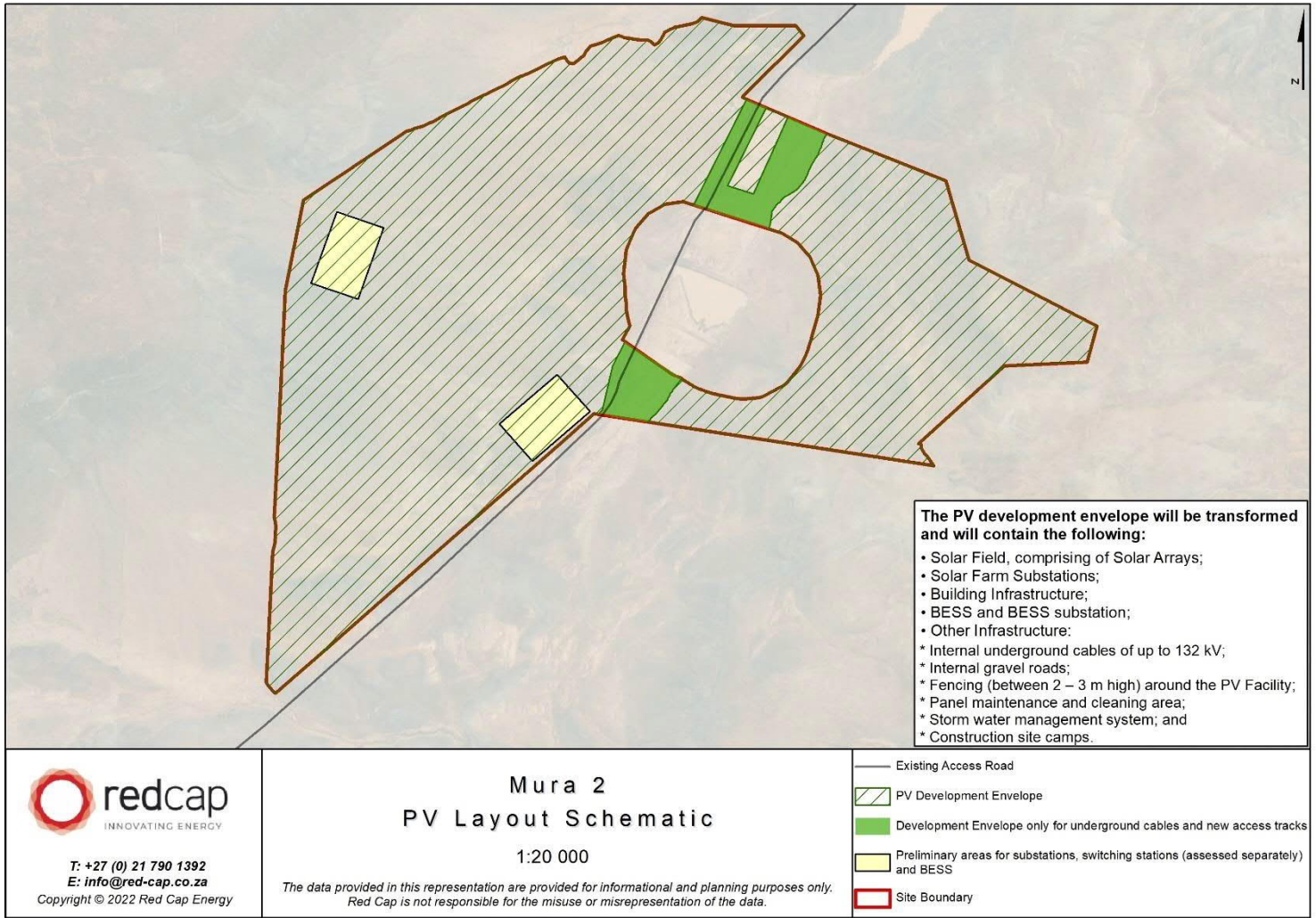
Figure 3-3 – Proposed Development Envelope for Mura 2 PV Facility
