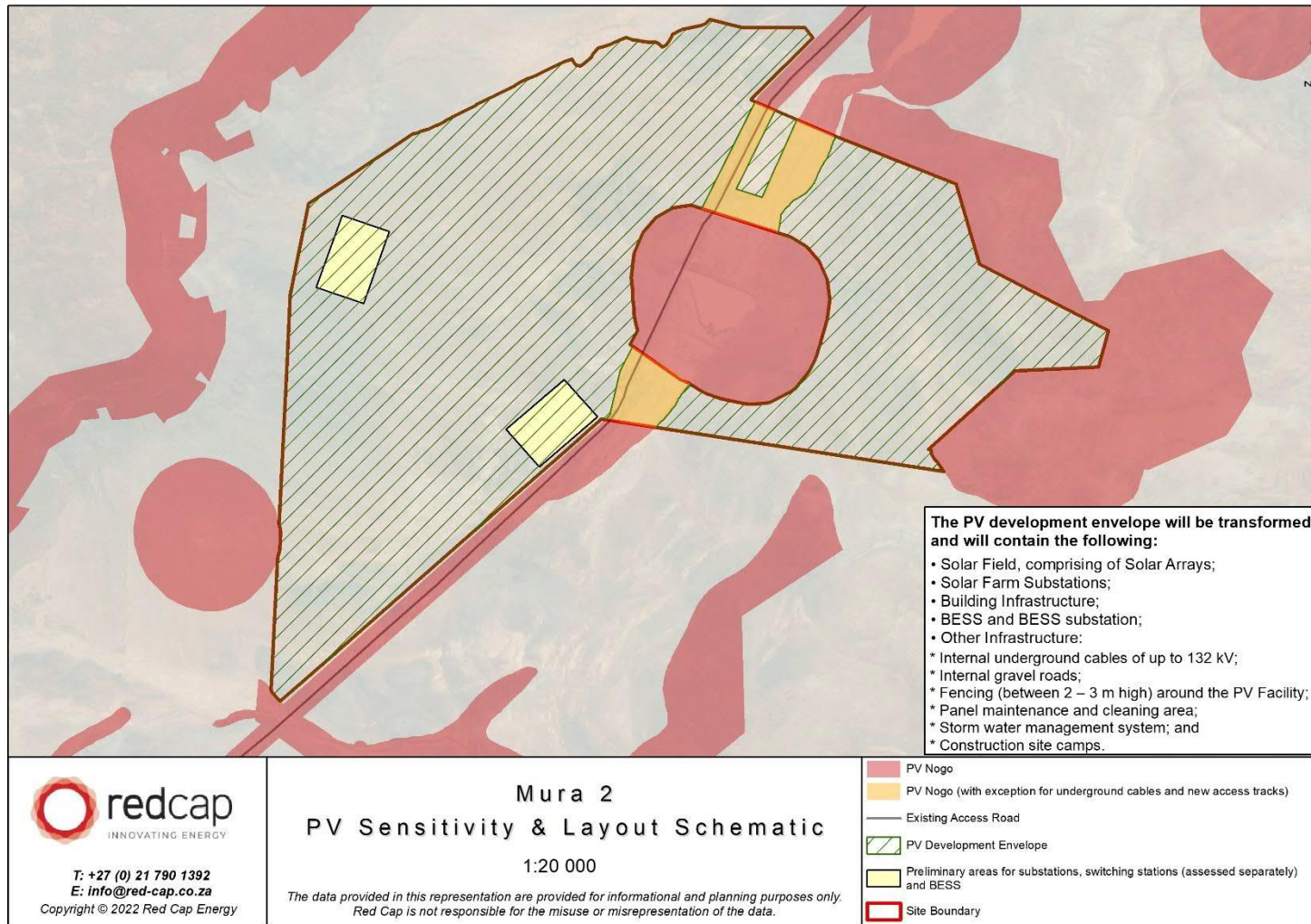
Figure 3-1 – Combined No-Go Sensitivity Map and Proposed Development Envelope for Mura 2 PV Facility
