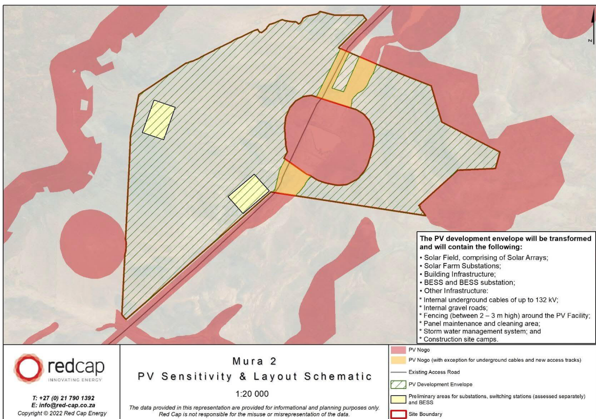
Figure 3: Combined No-Go Sensitivity Map and Proposed Development Envelope for Mura 2 PV Facility
