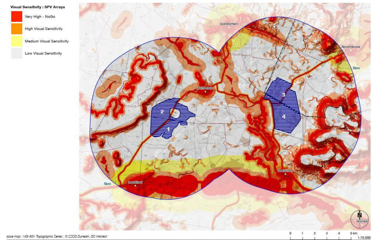
Figure 19: Visual Sensitivity
