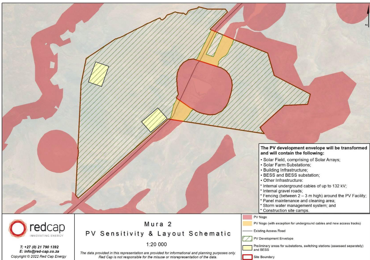
Figure 18: Combined No-Go Sensitivity Map for the Mura 2 Solar PV Facility
