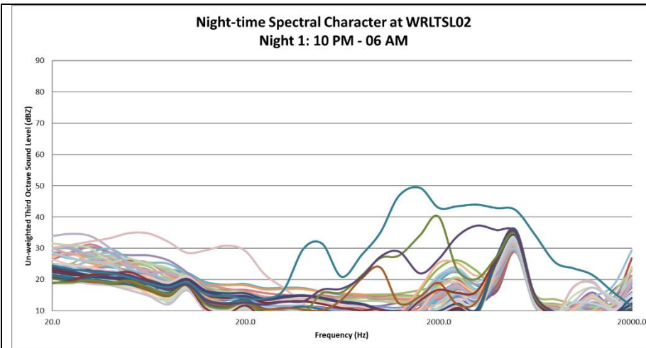
Figure 4-14: Night 1 spectral frequencies at WRLTSL02
