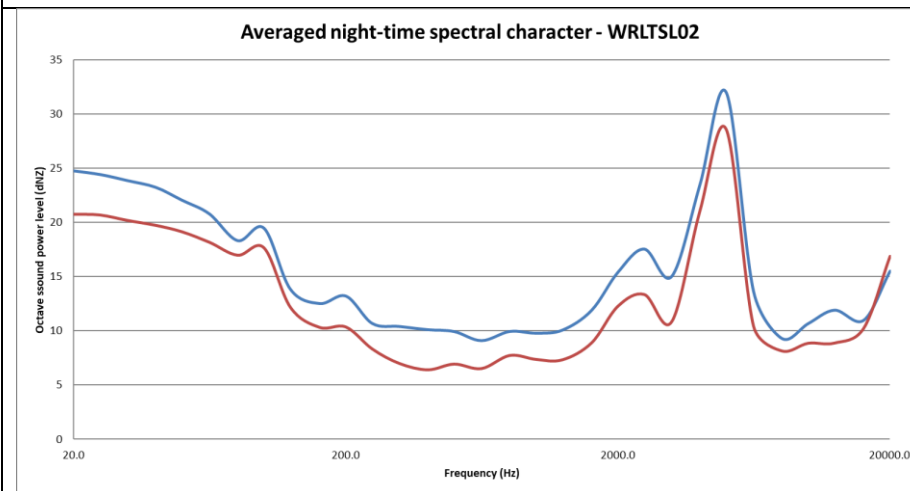
Figure 4-16: Average night-time frequencies at WRLTSL02
