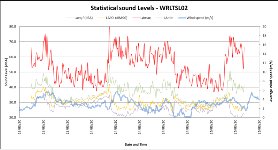
Figure 4-11: Maximum, minimum and statistical values at WRLTSL02
