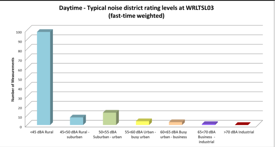
Figure 4-29: Classification of daytime measurements in typical noise districts at WRLTSL04
