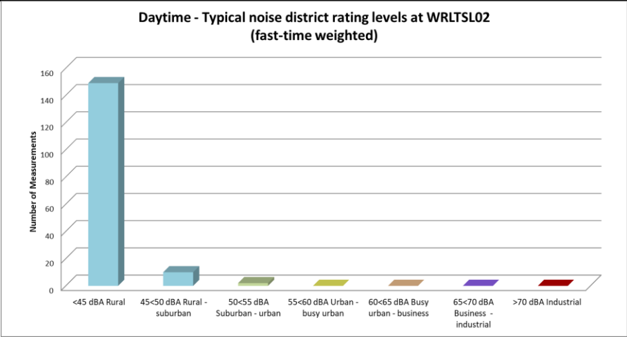
Figure 4-13: Classification of daytime measurements in typical noise districts at WRLTSL02
