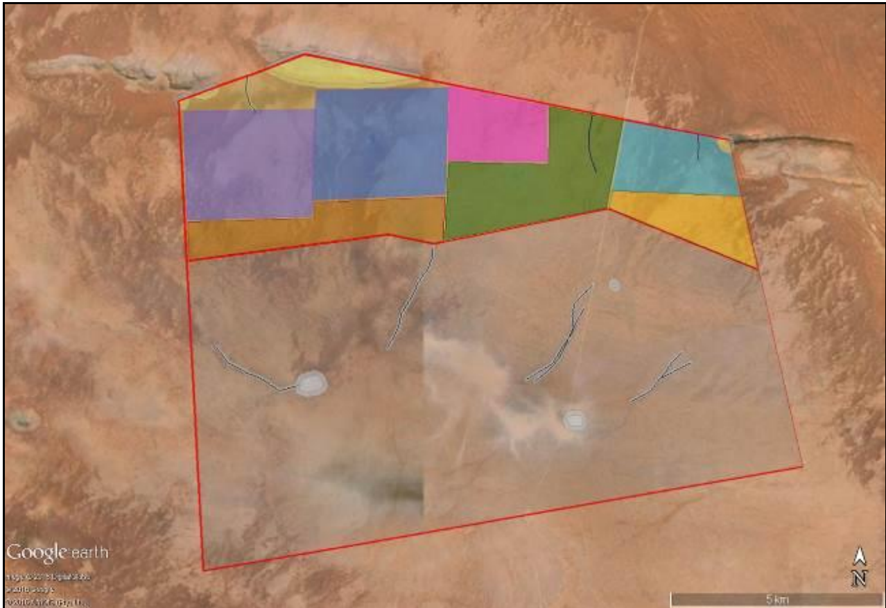
Figure 2: Close-up of the proposed layout. The CSP facilities are shown as purple and dark blue polygons, while the PV facilities are in dark orange, light orange, pink, green and light blue.
