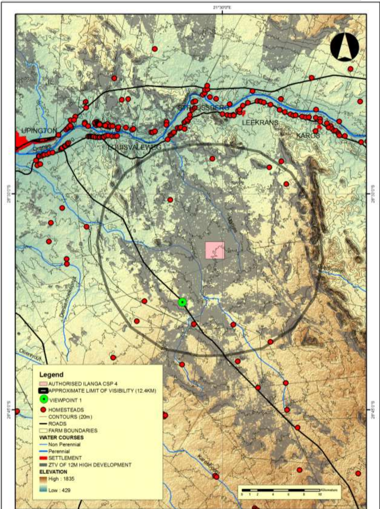
MAP 4: ZTV OF 12 M HIGH DEVELOPMENT ON AUTHORISED ILANGA CSP 4
