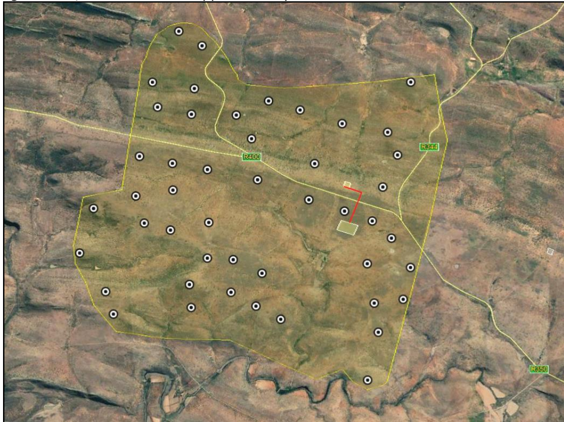
Figure 2: Aerial view of the development envelope indicating the proposed wind turbine layout (white dots), substation site (yellow rectangle) and power line (red line).
