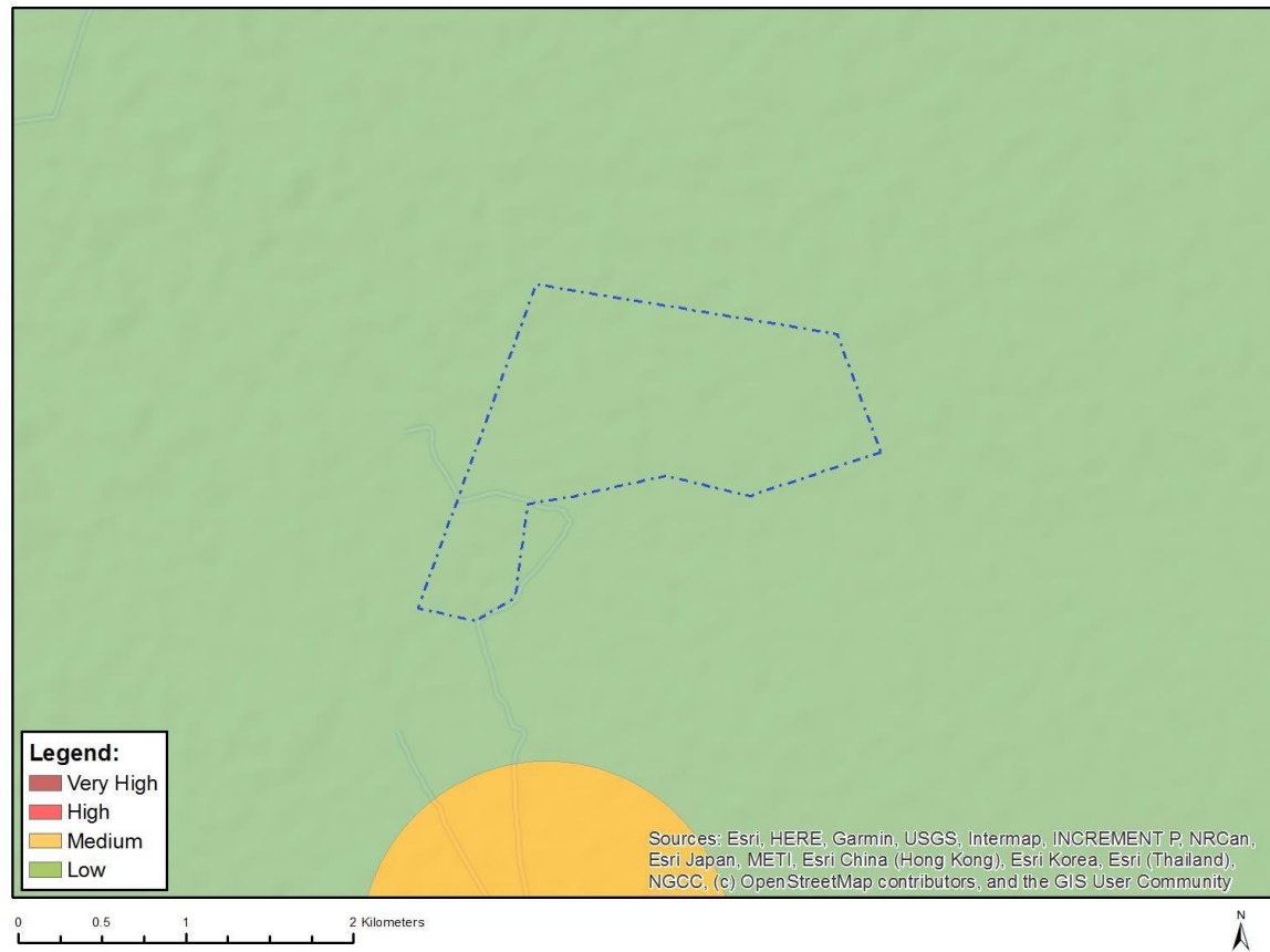
Figure 11: Map of relative RFI theme sensitivity
