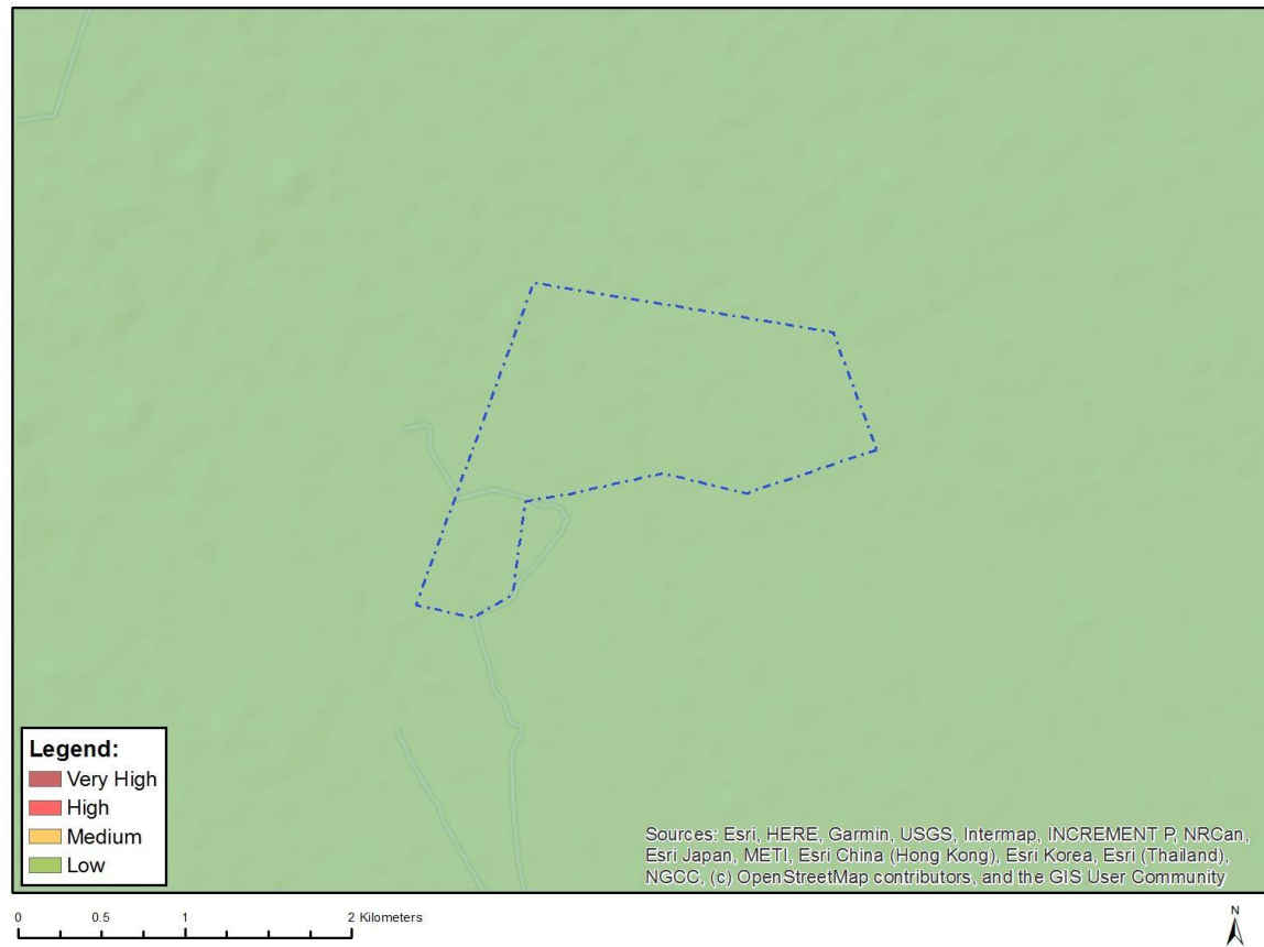
Figure 8: Map of relative defence theme sensitivity
