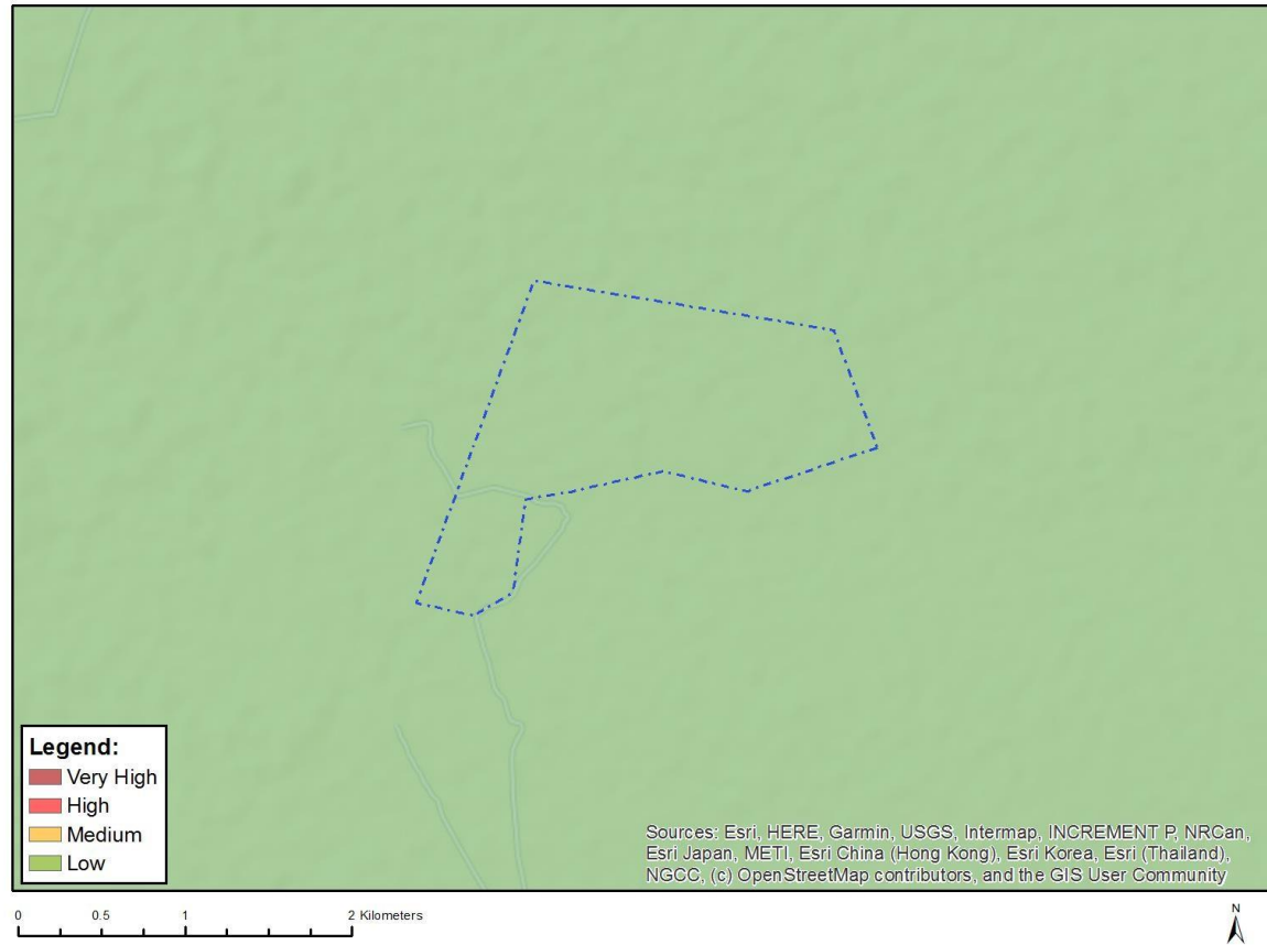
Figure 7: Map of relative civil aviation theme sensitivity
