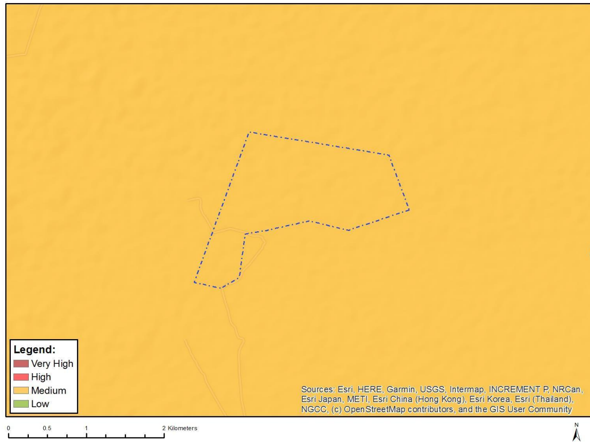
Figure 10: Map of relative plant species theme sensitivity
