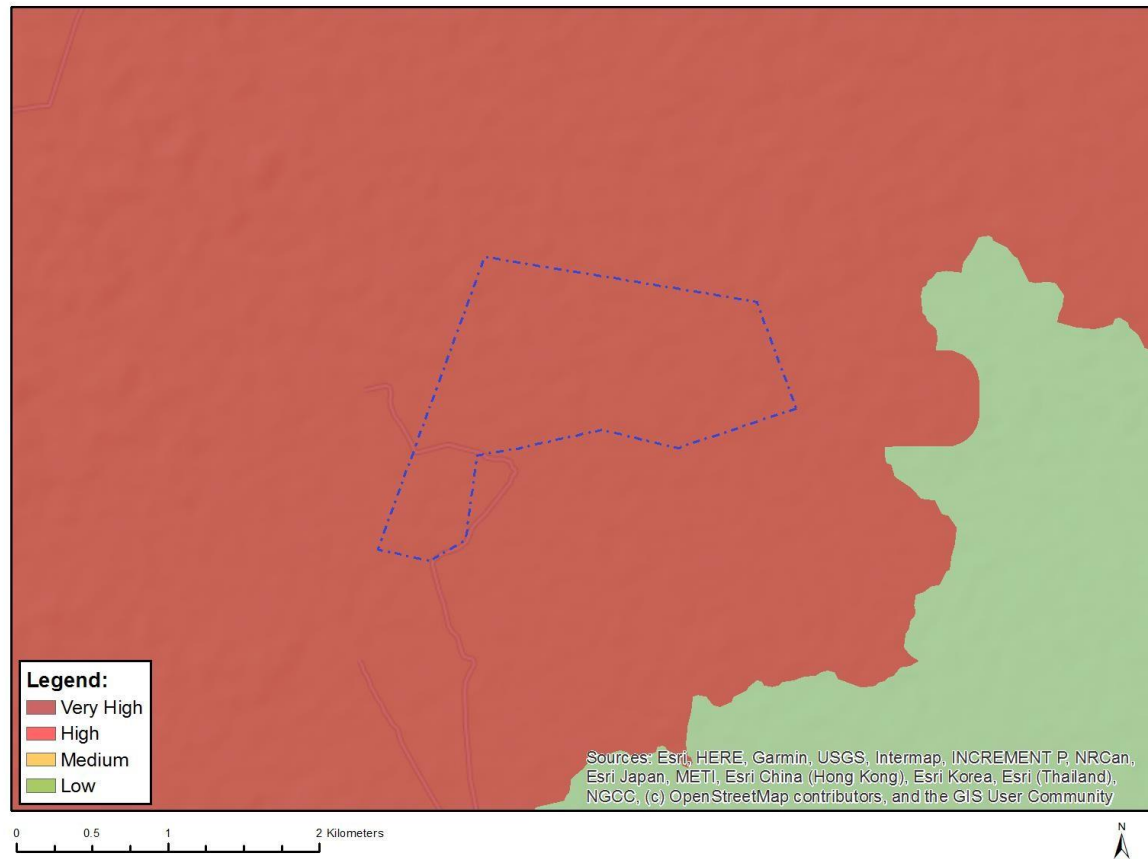
Figure 12: Map of relative terrestrial biodiversity theme sensitivity
