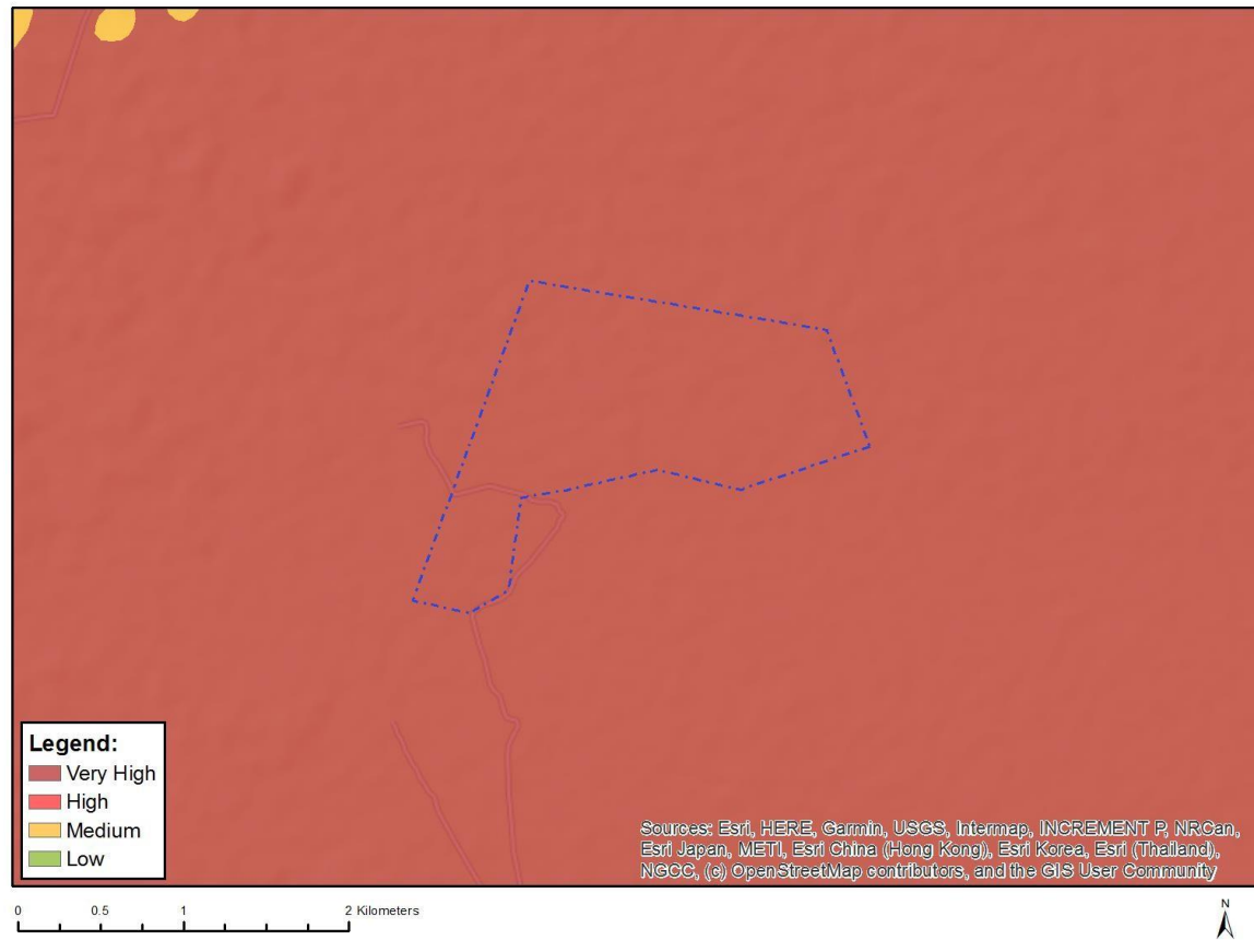
Figure 9: Map of relative palaeontology theme sensitivity
