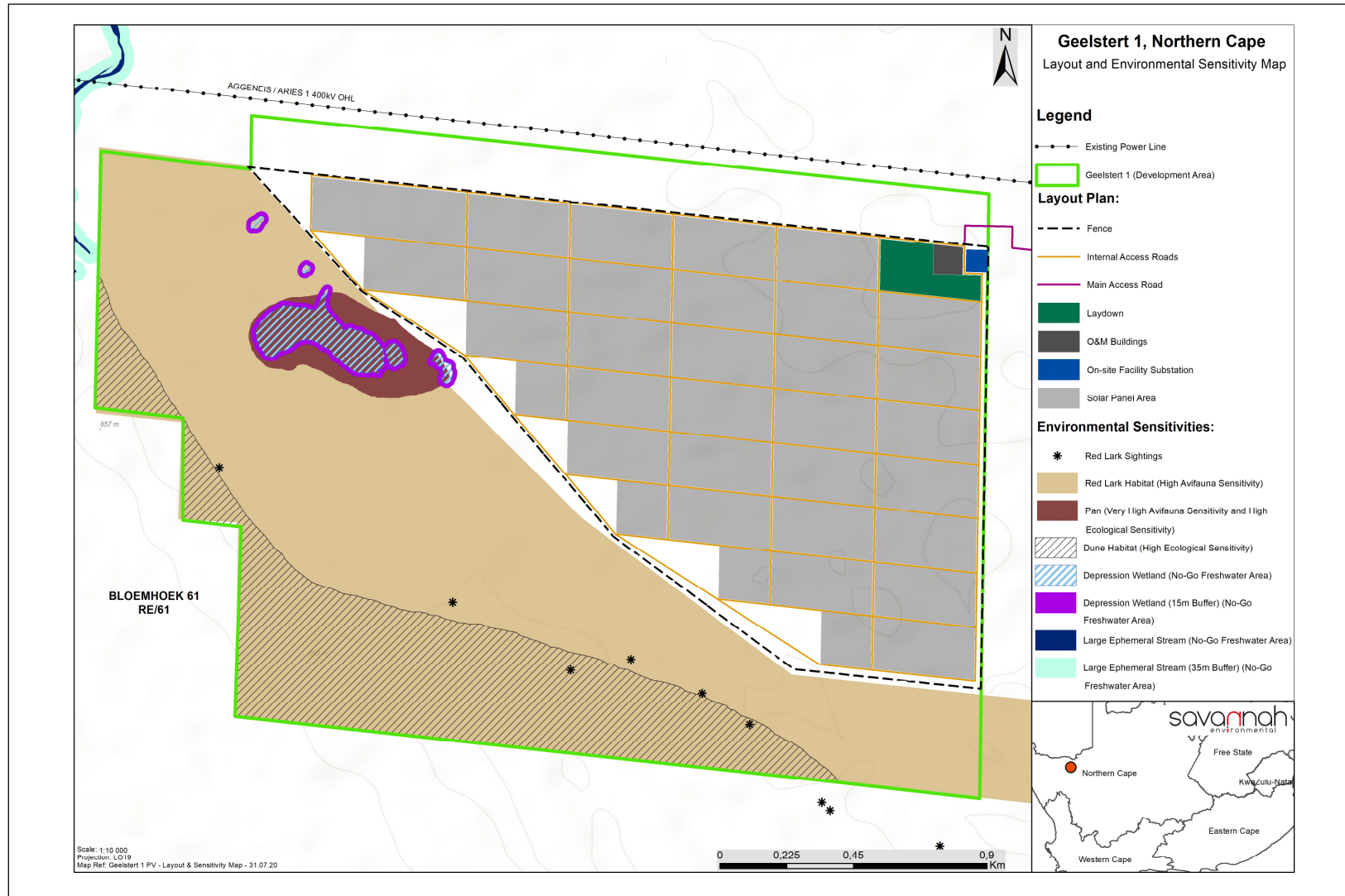
Figure 2.3: Preferred layout map of the preferred development footprint for Geelster 1, as was assessed as part of the BA process, overlain with the environmental sensitivities.
