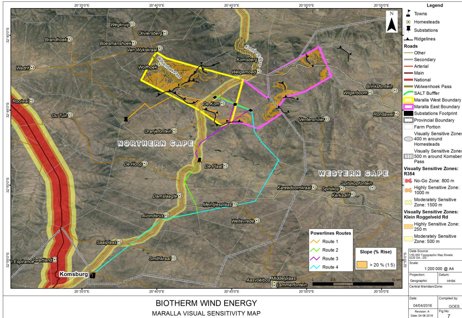
Figure 3: Visual Sensitivity Map: Maralla West and East
