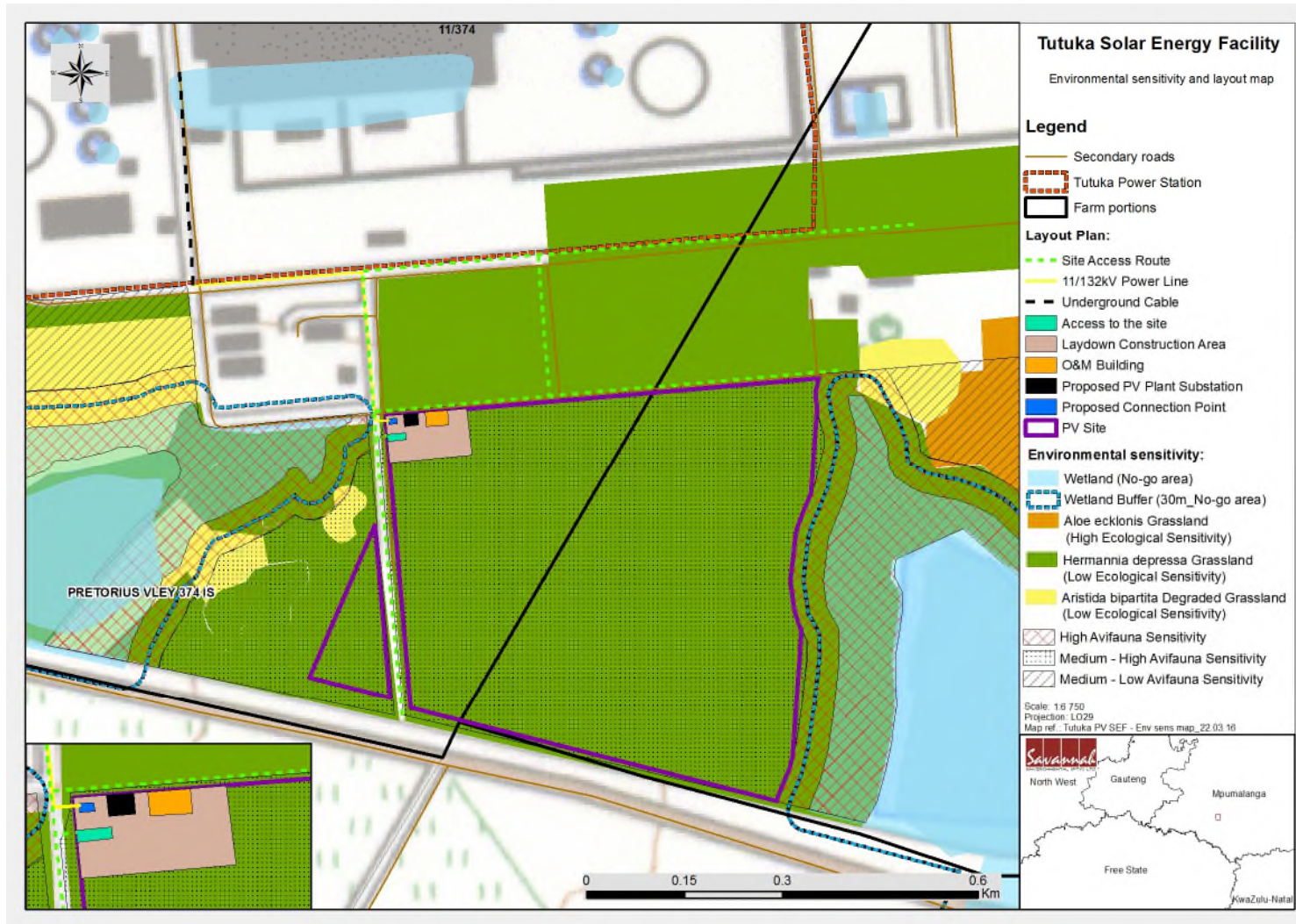
Figure 2.2: The final/optimised layout map superimposed (overlain) on the environmental sensitivity for the Tutuka PV Solar Energy Facility
