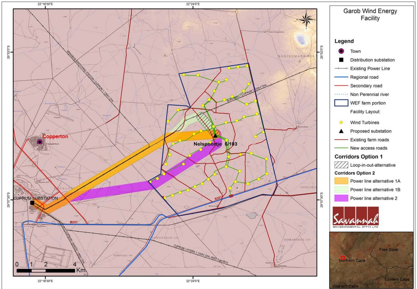
Figure 4. Power line corridors and turbine positions as indicated by Savannah.
