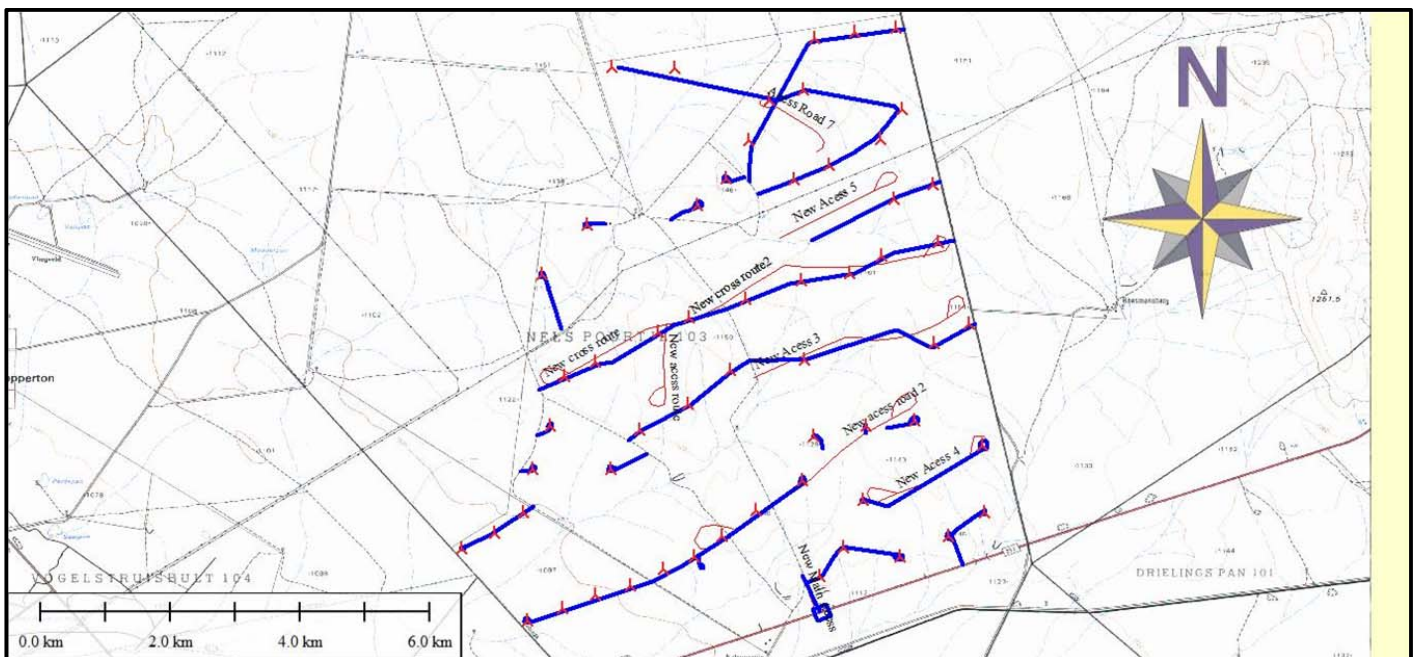
Figure 6. New turbine positions and access roads (blue) in relation to the old access routes (red).
