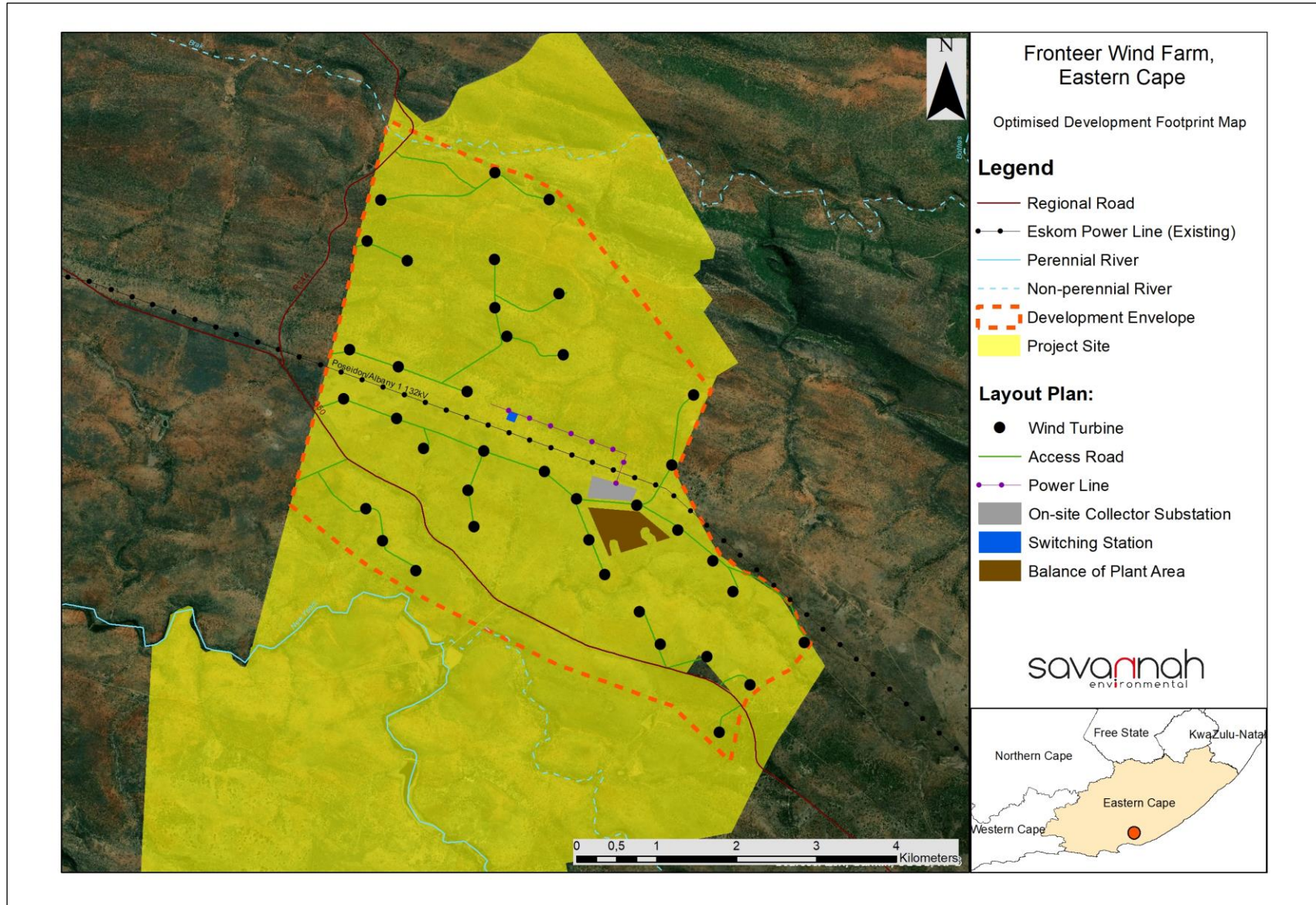
Figure 2.3: Final preferred (optimised) development footprint for the Fronteer Wind Farm considered to be acceptable for development (refer to Appendix A for A3 maps).
