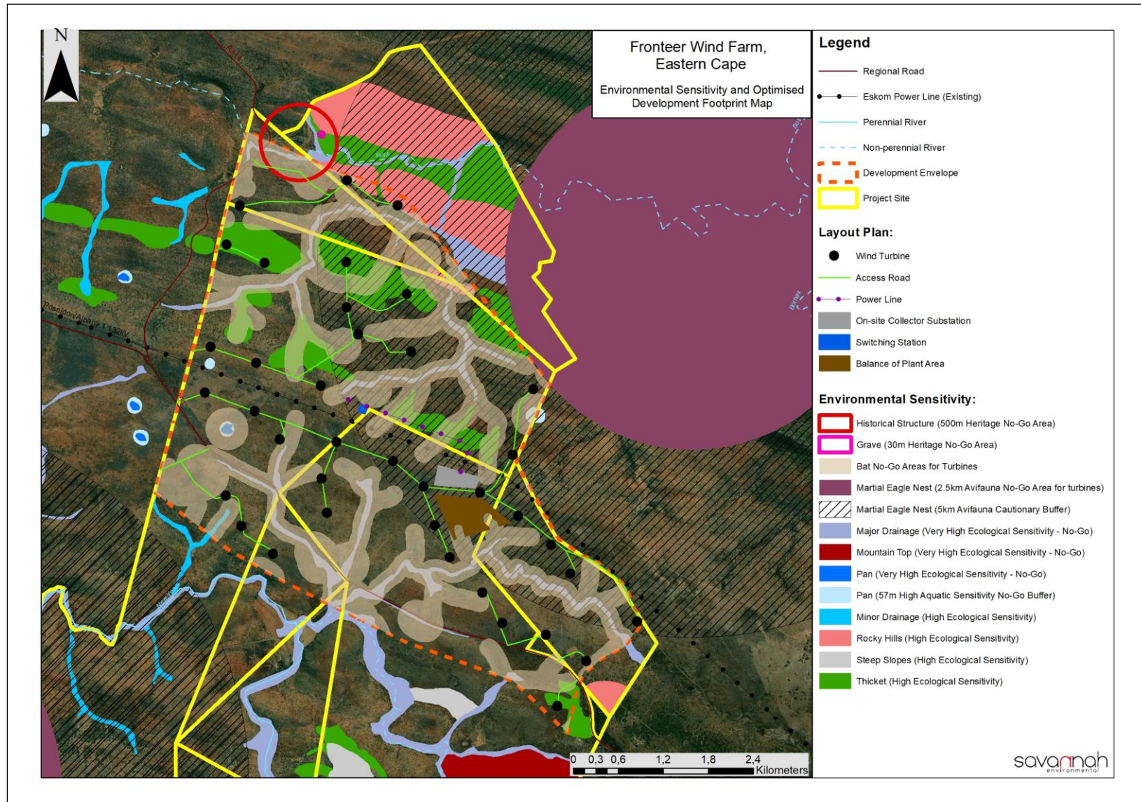
Figure 2.2: Final preferred (optimised) development footprint (~49.4ha) for the Fronteer Wind Farm, overlain with the identified environmental sensitivities (refer to Appendix A for A3 maps).
