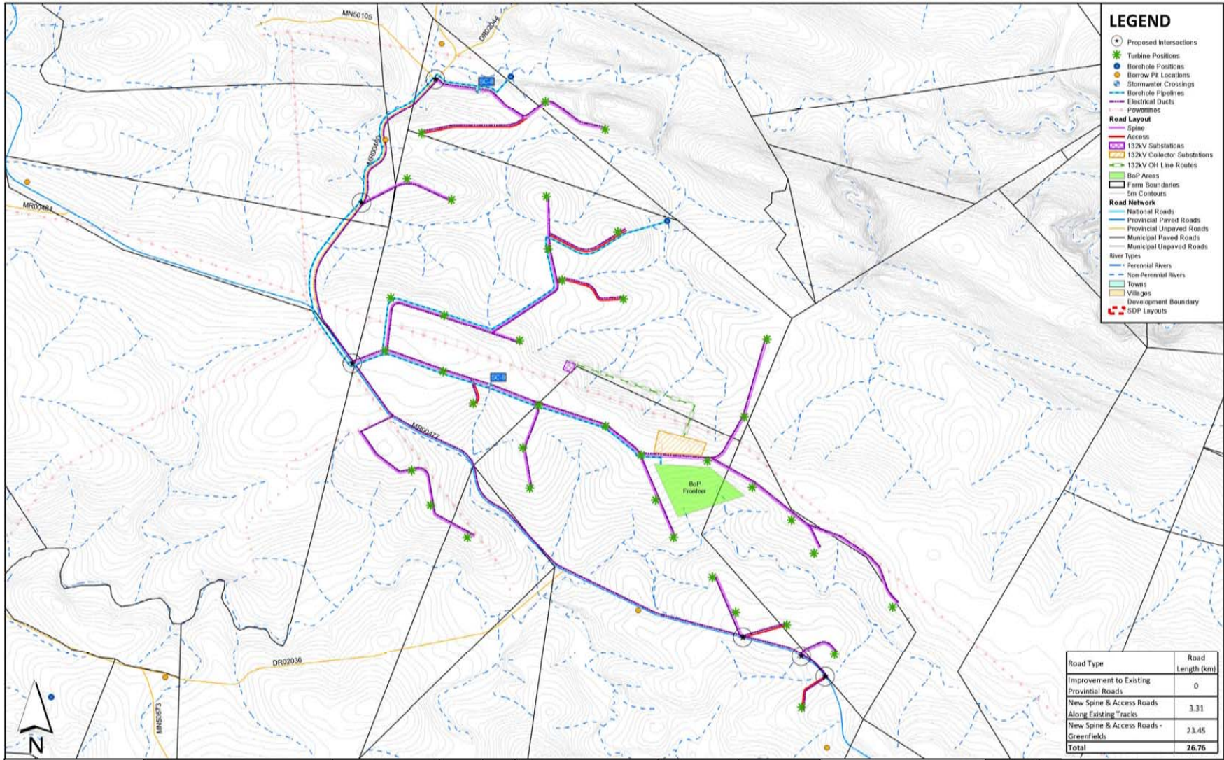
Figure 2 – Frontier Layout Plan
