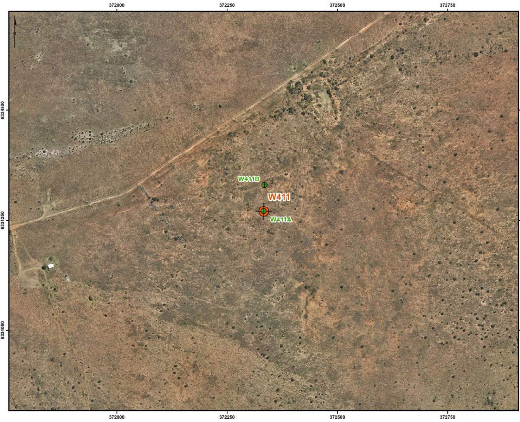
Figure 6: Borehole W411
