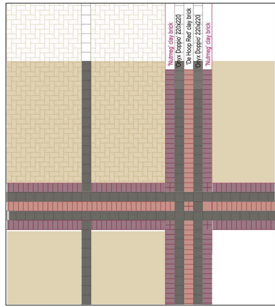
Typical Band Pattern for the Central Plaza 1:50
