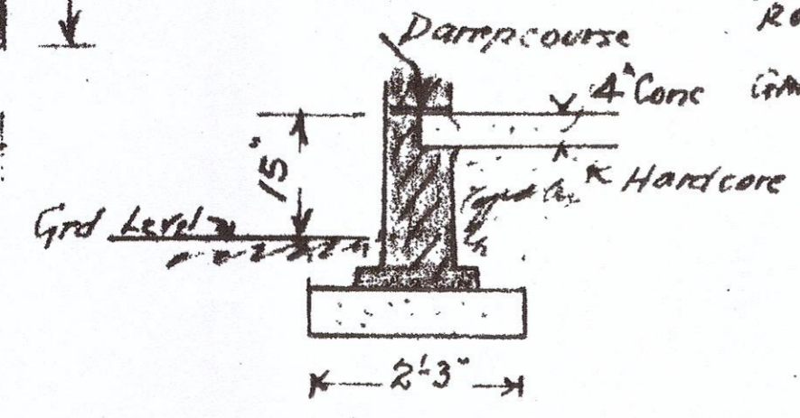
SECTION THROUGH WALL
