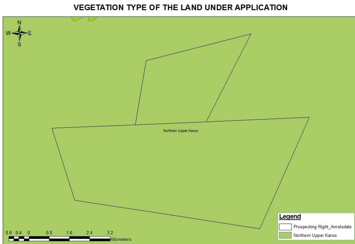
Figure 2: Vegetation type of the area under application.
