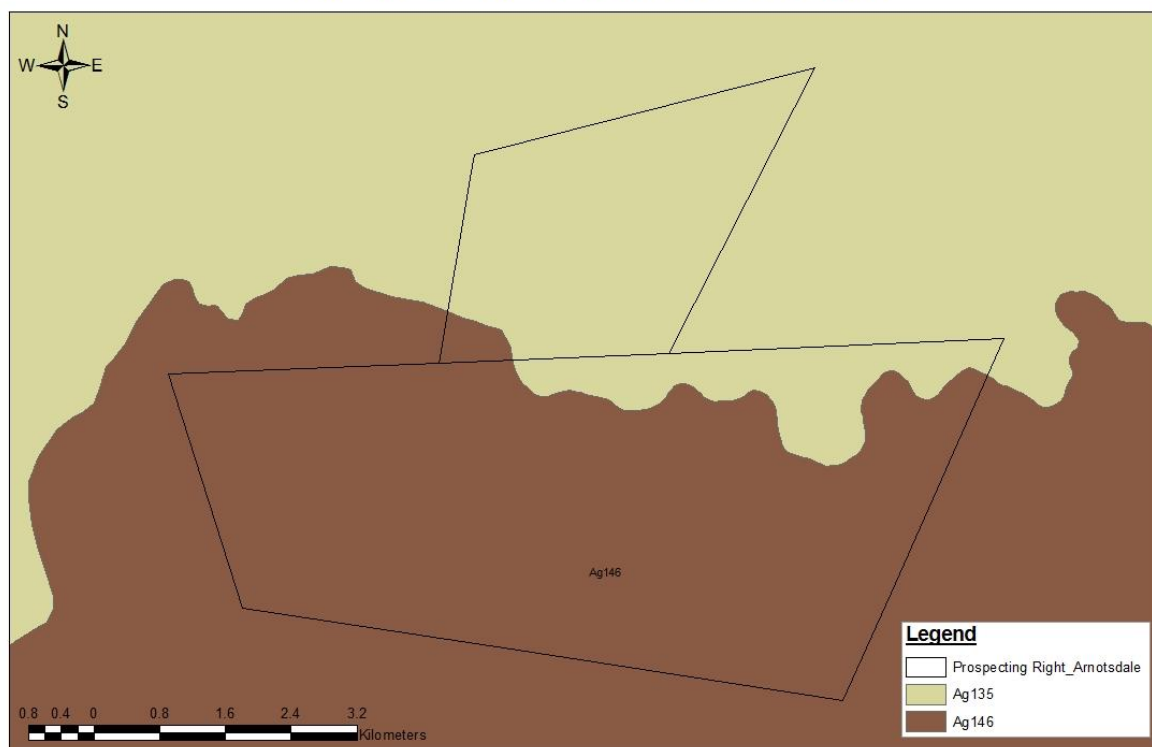
Figure 1: Soil types of the area under application.
