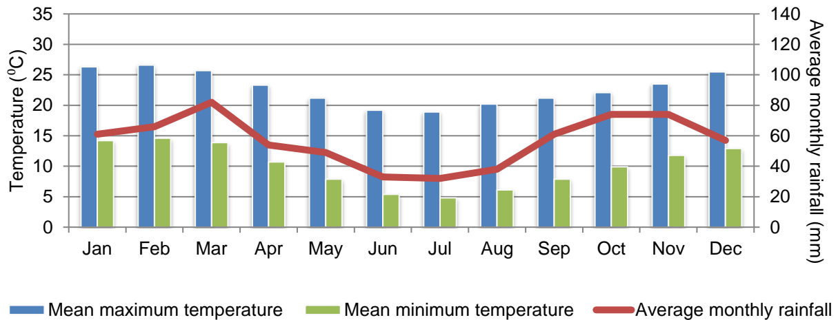
Figure 4: Average monthly maximum and minimum temperature at Grahamstown. The average monthly rainfall is in mm (SAWS, 1998)
