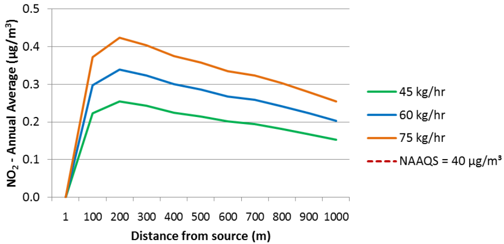
Figure 8: Predicted 1-hour average (top) and annual average (bottom) NO 2 ambient concentrations in µg/m 3 resulting from emissions from the incinerator in isolation
