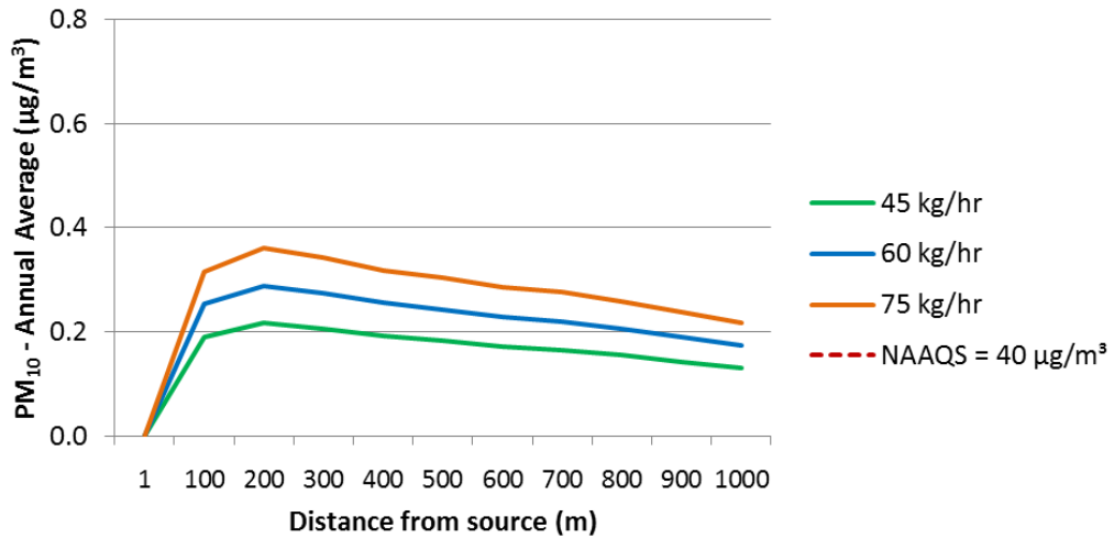
Figure 6: Predicted 24-hour average (top) and annual average (bottom) PM 10 ambient concentrations in µg/m 3 resulting from emissions from the incinerator in isolation
