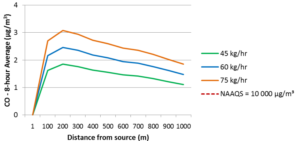
Figure 10: Predicted 1-hour average (top) and 8-hour average (bottom) CO ambient concentrations in \mu\text{g}/\text{m}^3 resulting from emissions from the incinerator in isolation
