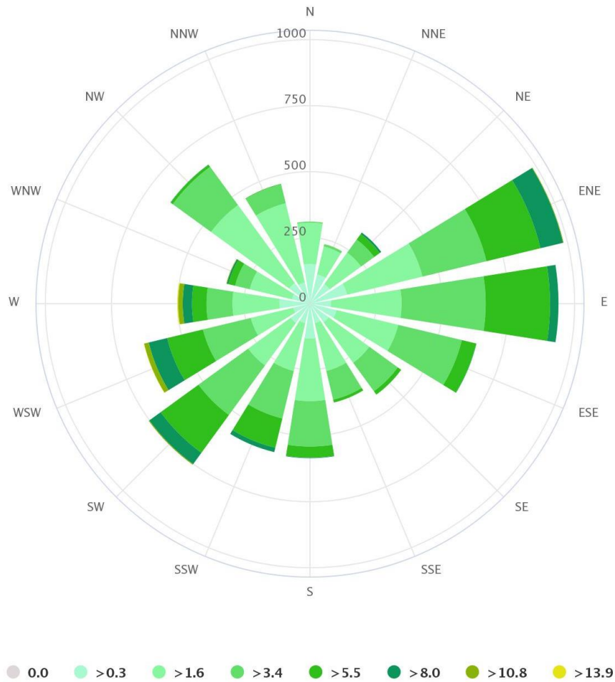
Figure 5: Annual windrose at Grahamstown with wind speed in m/s and frequency bands of 500 hours https://www.meteoblue.com/en/weather/forecast/modelclimate
