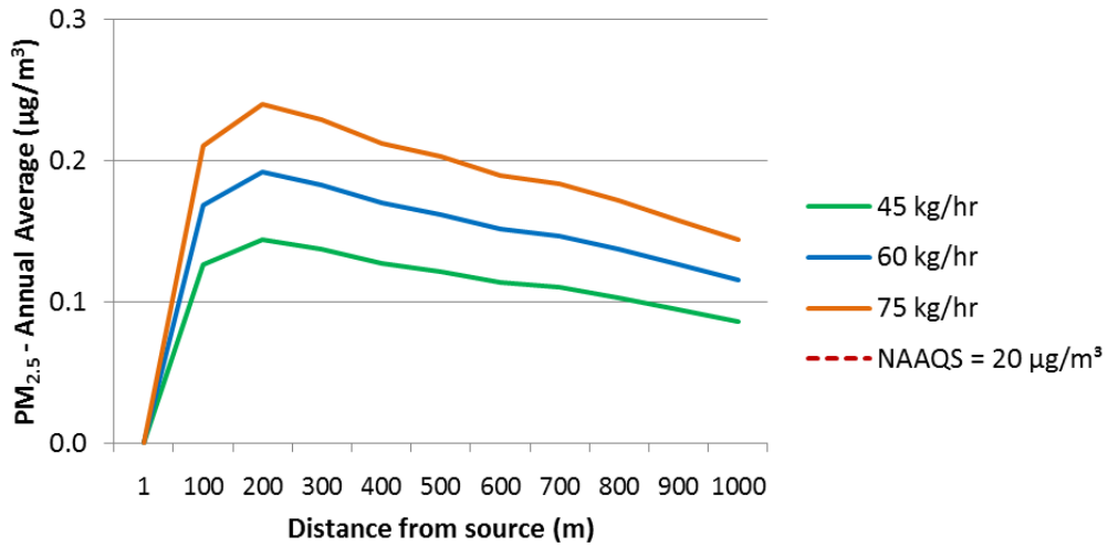
Figure 7: Predicted 24-hour average (top) and annual average (bottom) PM 2.5 ambient concentrations in µg/m 3 resulting from emissions from the incinerator in isolation
