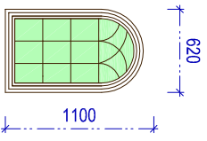
W3 Small paned wooden window (non opening)
