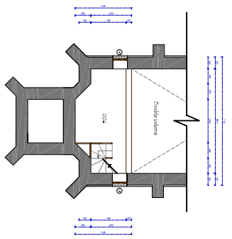
SECOND FLOOR PLAN 1:300 Garrison Church
