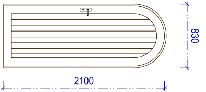
D2 Brace & ledge door with tongue & groove battens (open back) and wooden frame
