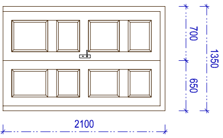
W1 Small paned vertical sliding sash wooden window
