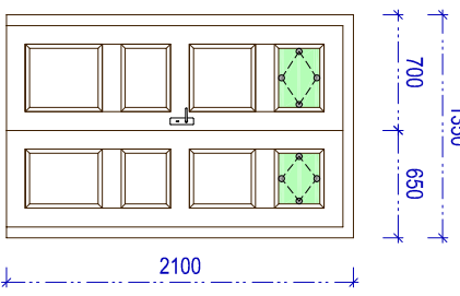
D3 Custom folded panel wooden double door with pivoting glass panels and wooden doorframe
