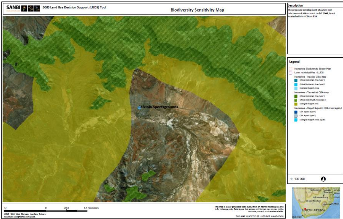
Figure 8: SANBI BGIS Biodiversity Map. The proposed site is not located within an CBA or ESA.
