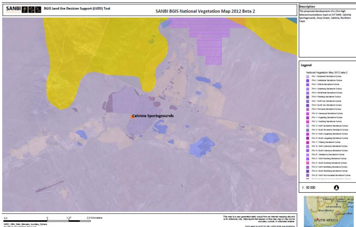
Figure 9: SANBI BGIS map showing the vegetation cover of the area. The site is indicated by the orange dot.
