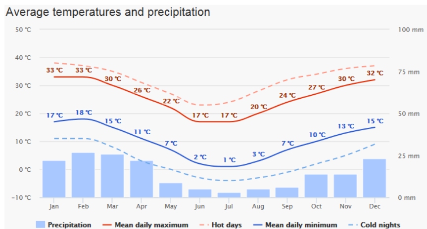
Figure 5 – Average temperatures and precipitation of the Copperton area
