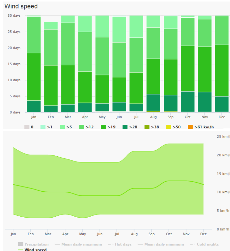
Figure 4 – Wind speed of the Copperton area
