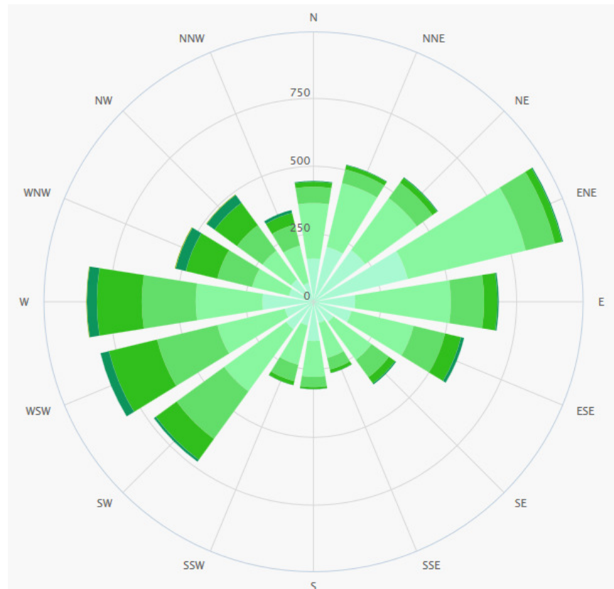
Figure 3 – Wind rose for Copperton area
