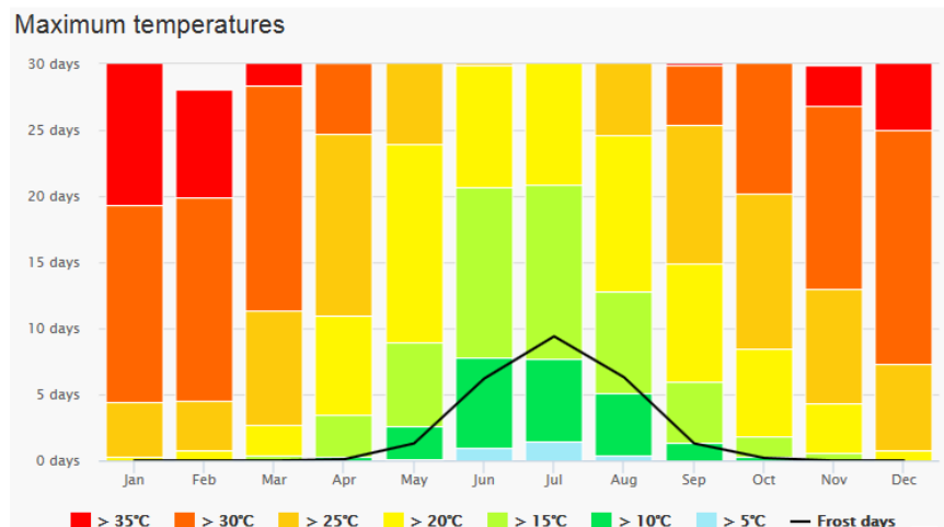
Figure 7 – Maximum temperatures in the Copperton area
