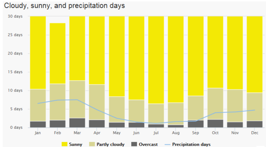
Figure 6 – Cloudy, sunny and precipitation days in the Copperton area
