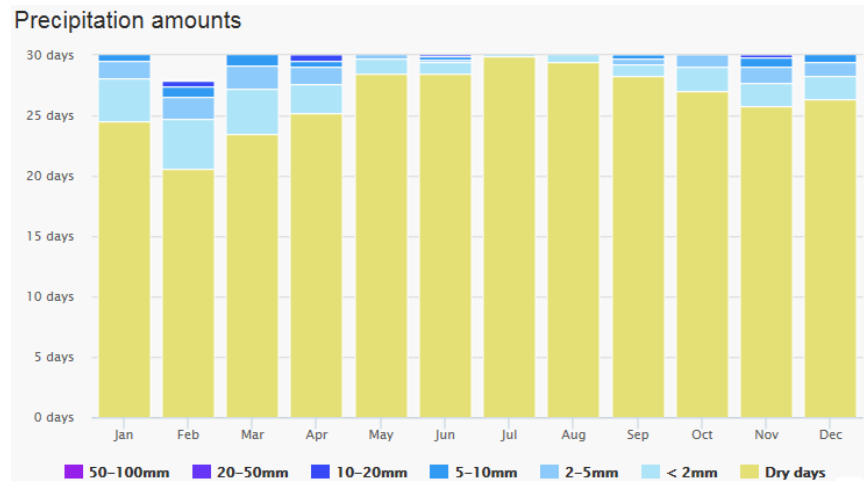
Figure 8 – Precipitation of the Copperton area
