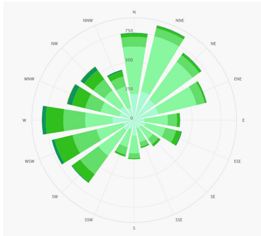
Figure 3 – Wind rose for Prieska area
