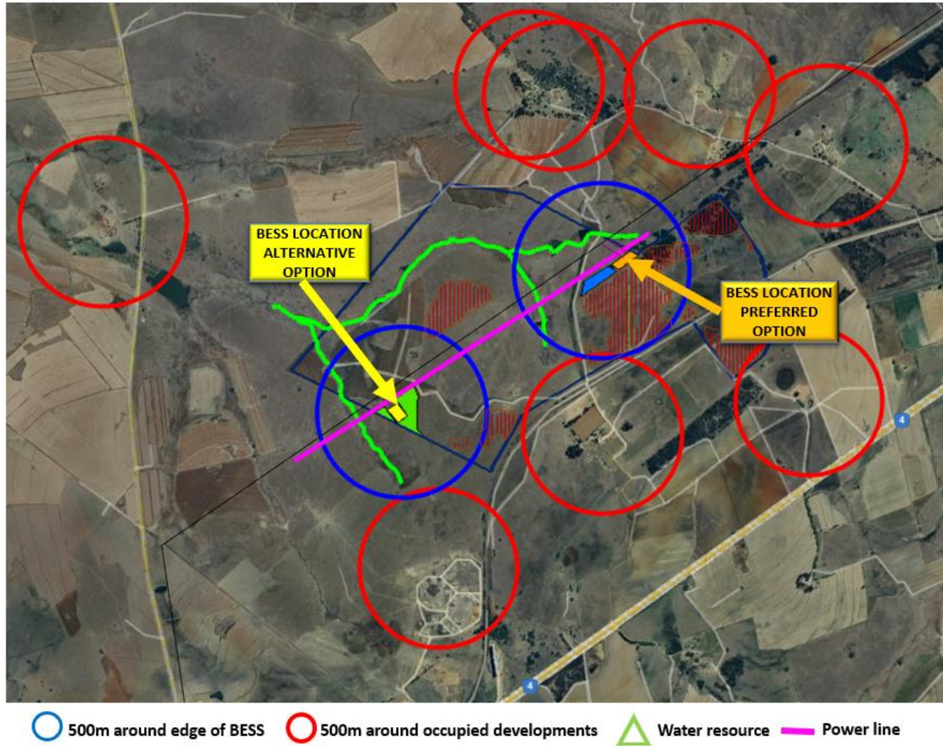
Figure 2.1.3 – 500m circles around the BESS Facilities (Blue) and Location of Occupied Developments / Farmhouses (Red) and Nearby Water Courses/Bodies (Green) in the immediate vicinity of the BESS
