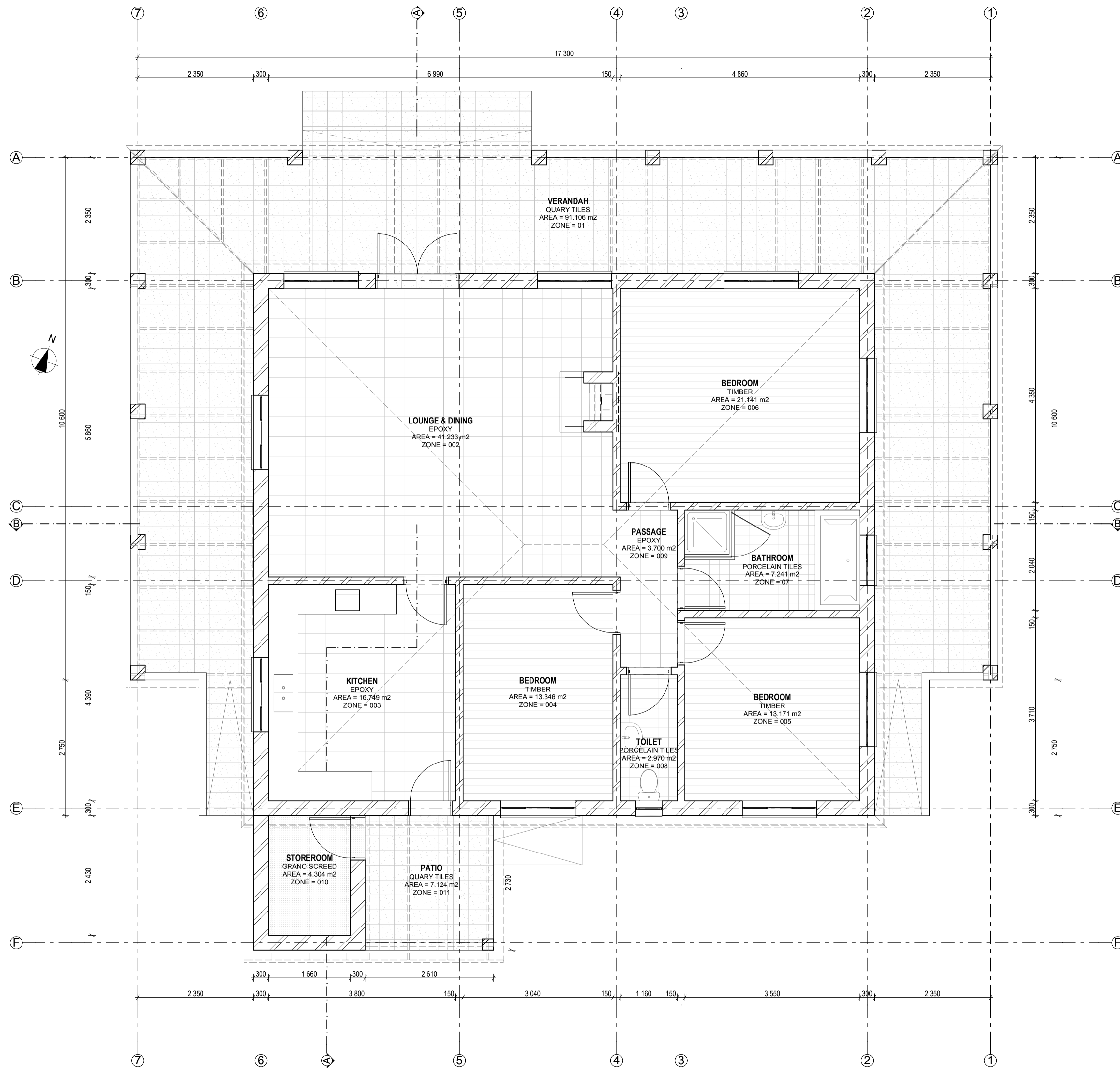
0. FLOOR FINISHES LAYOUT 1:50
