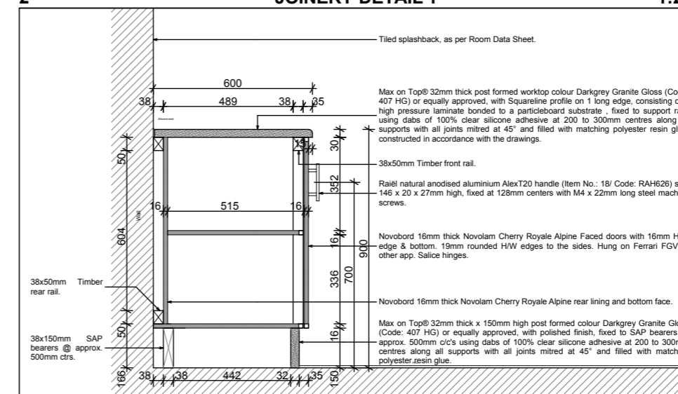
2 JOINERY DETAIL 2 1:20
