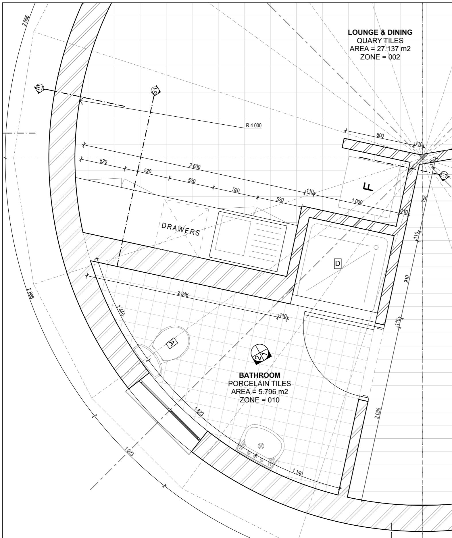
0. BATHROOM & KITCHEN LAYOUT 1:25
