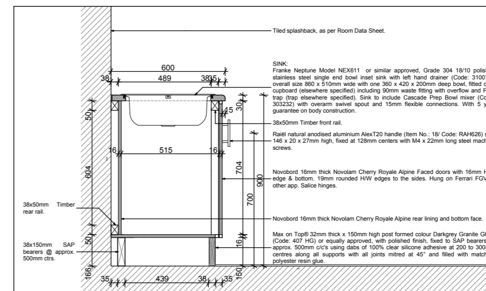
2 JOINERY DETAIL 1 1:20
