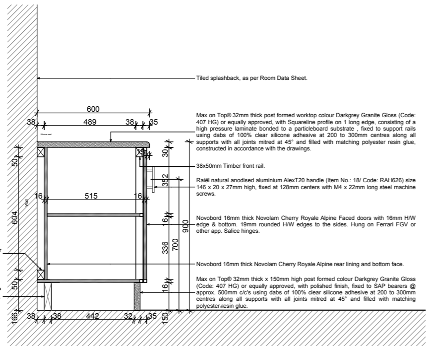
5 JOINERY DETAIL 1 1:20
