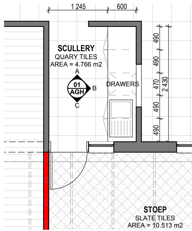
1 KITCHEN LAYOUT 1:50
