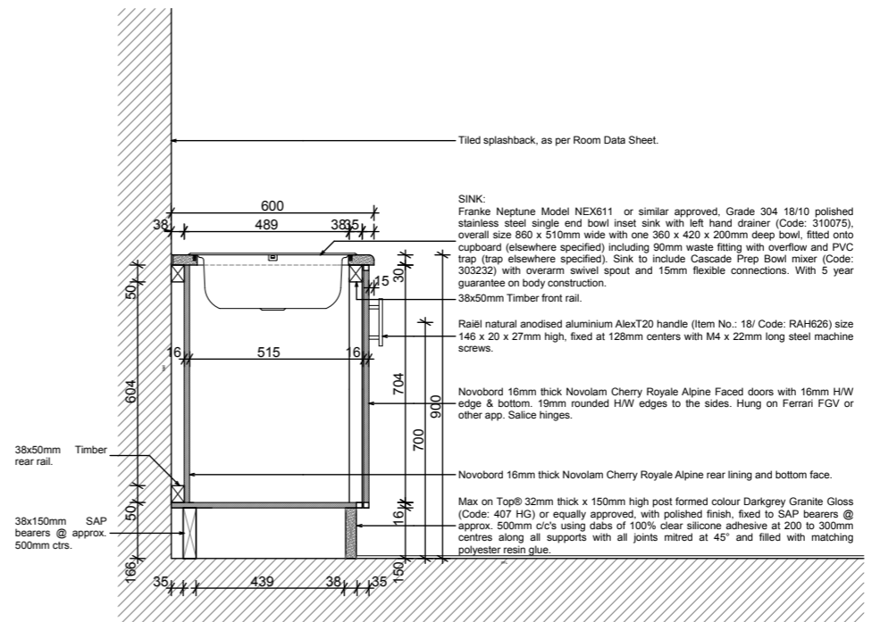
6 JOINERY DETAIL 2 1:20
