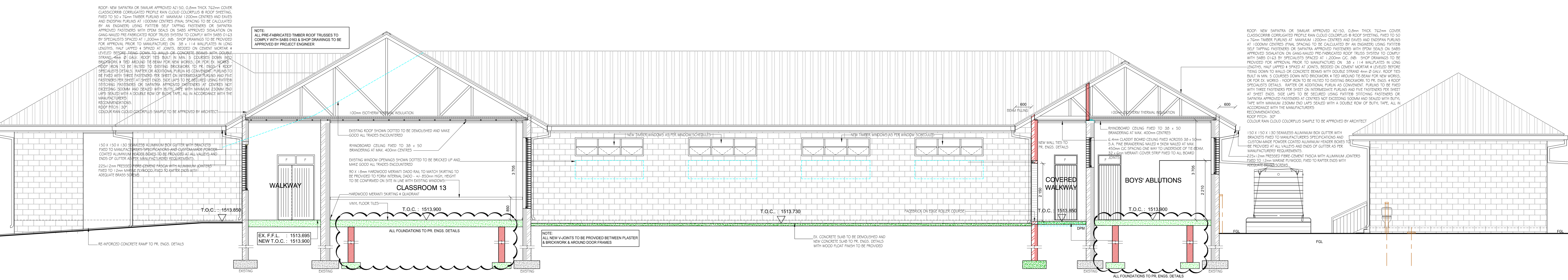
SECTIONAL ELEVATION L - L SCALE : 1 : 50
