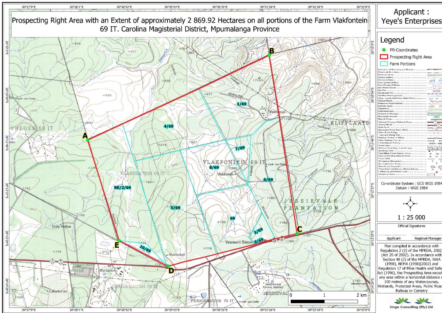
Figure 1: Regulation 2.2 plan of the proposed project area
