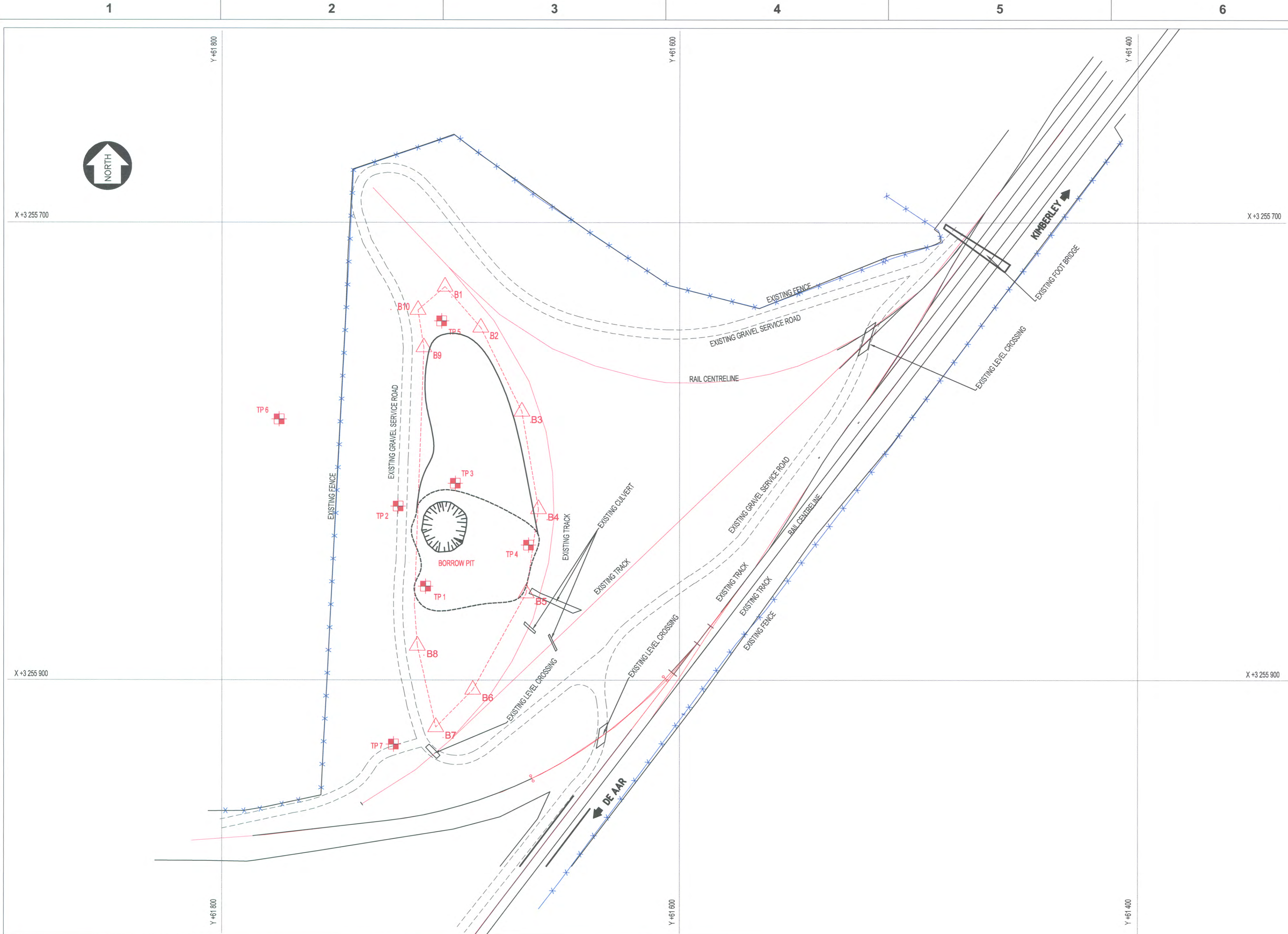
LAYOUT SCALE 1:1000
