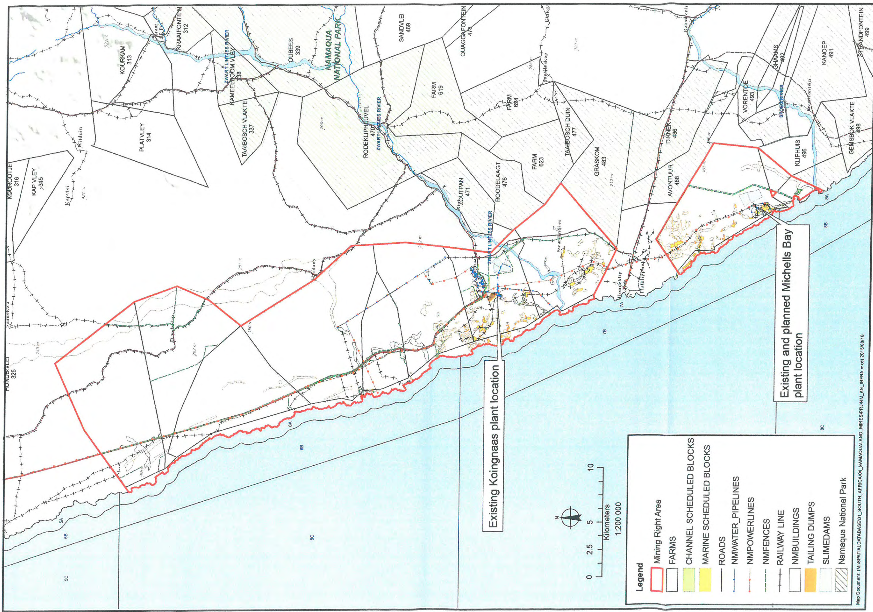
Appendix 4.3: Existing and planned infrastructure network
