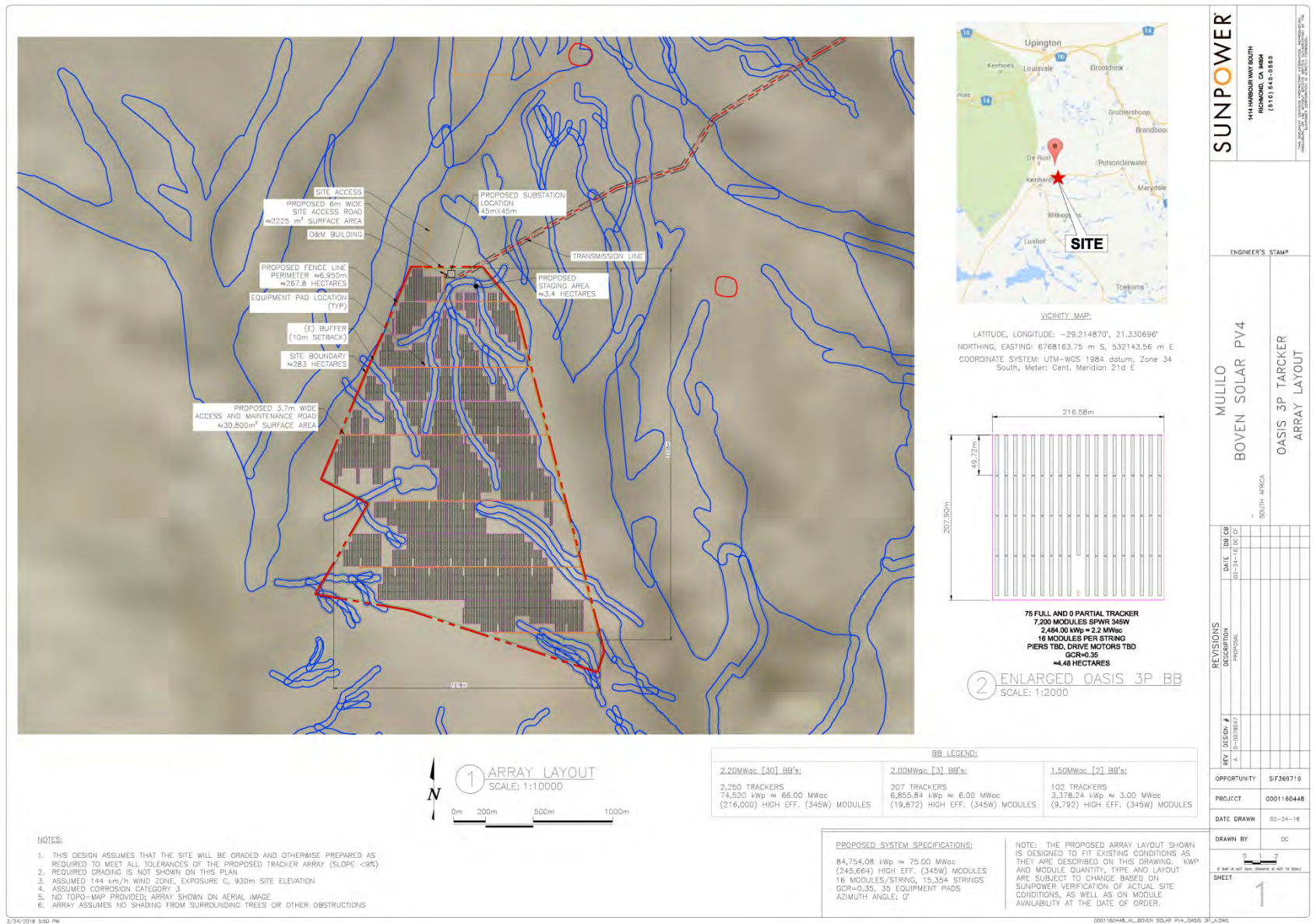
Figure 17.3: Layout for the proposed Boven Solar PV4 Facility.
