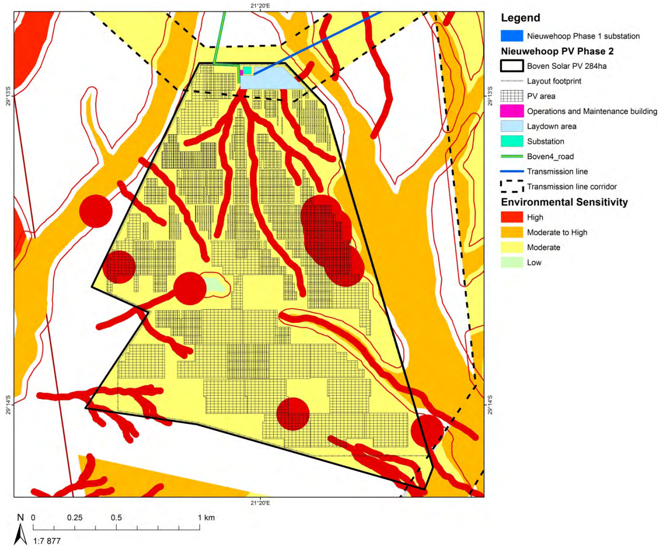
Figure 17.4: Combined layout and sensitivity map for the proposed Boven Solar PV4 Facility.
