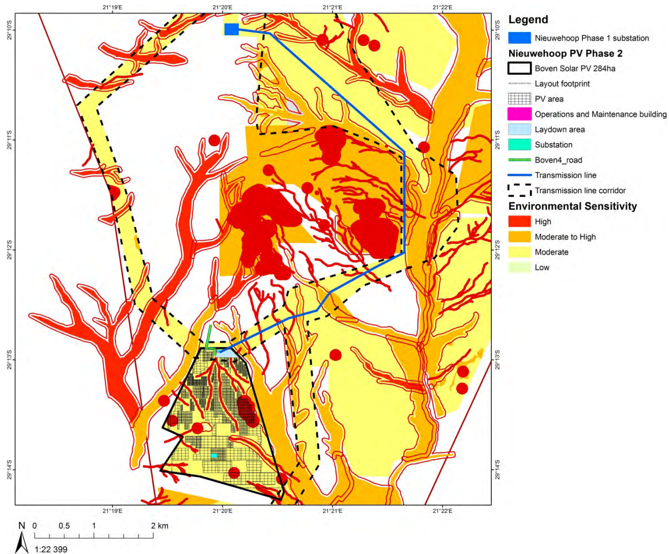
Figure 17.4: Combined layout and sensitivity map for the proposed Boven Solar PV4 Facility (including powerline).
