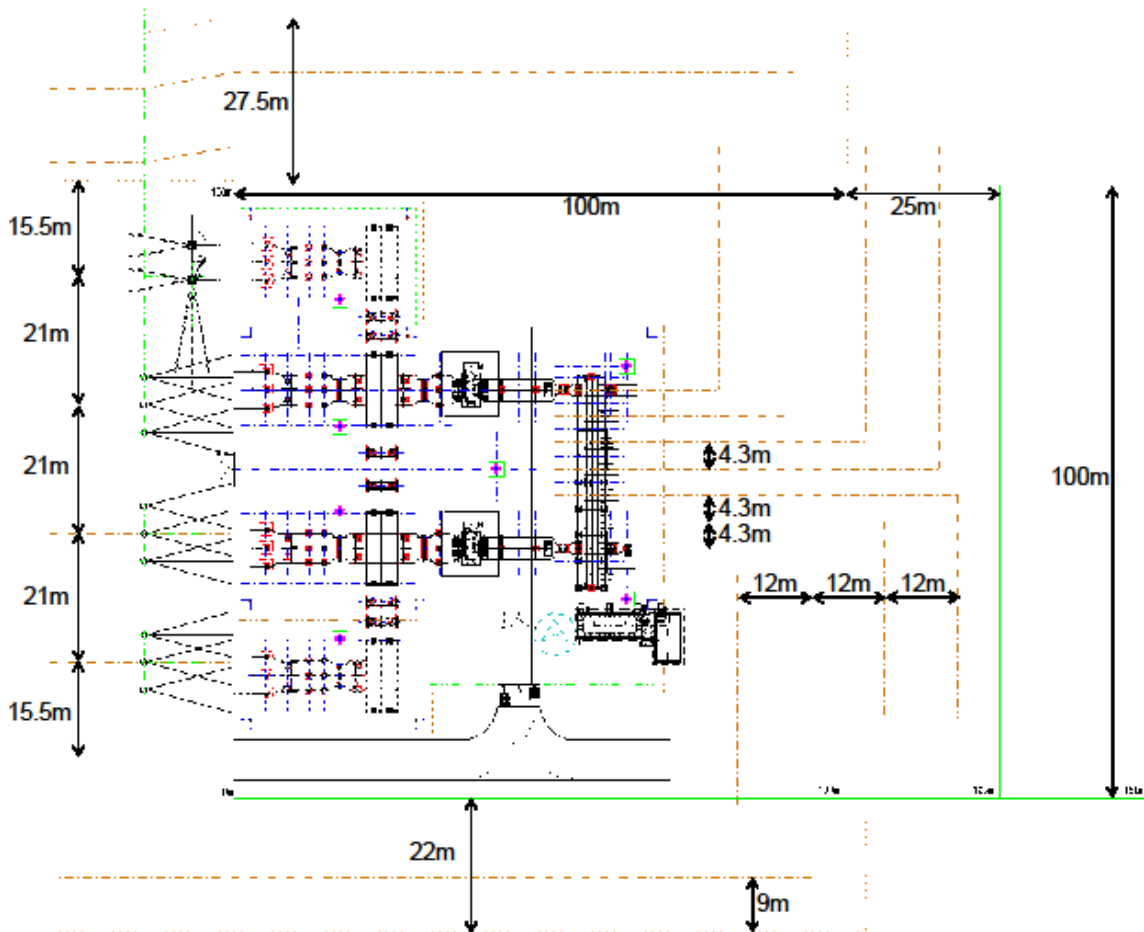
Typical substation site layout and line routes
