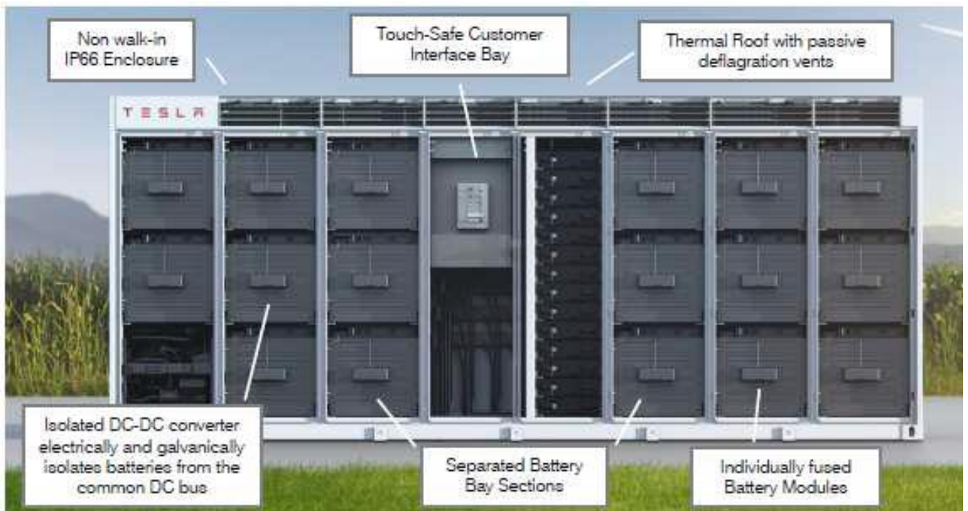
Typical Battery Modules in a BESS with the Separated Sections
