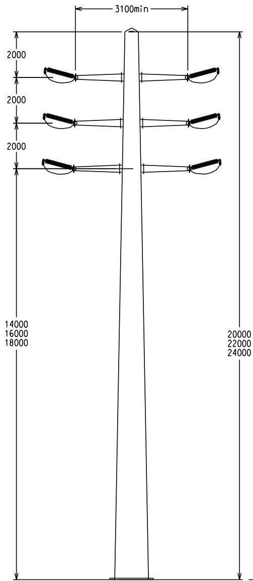
STRAIN STRUCTURE 15°/30°/45°/60°
