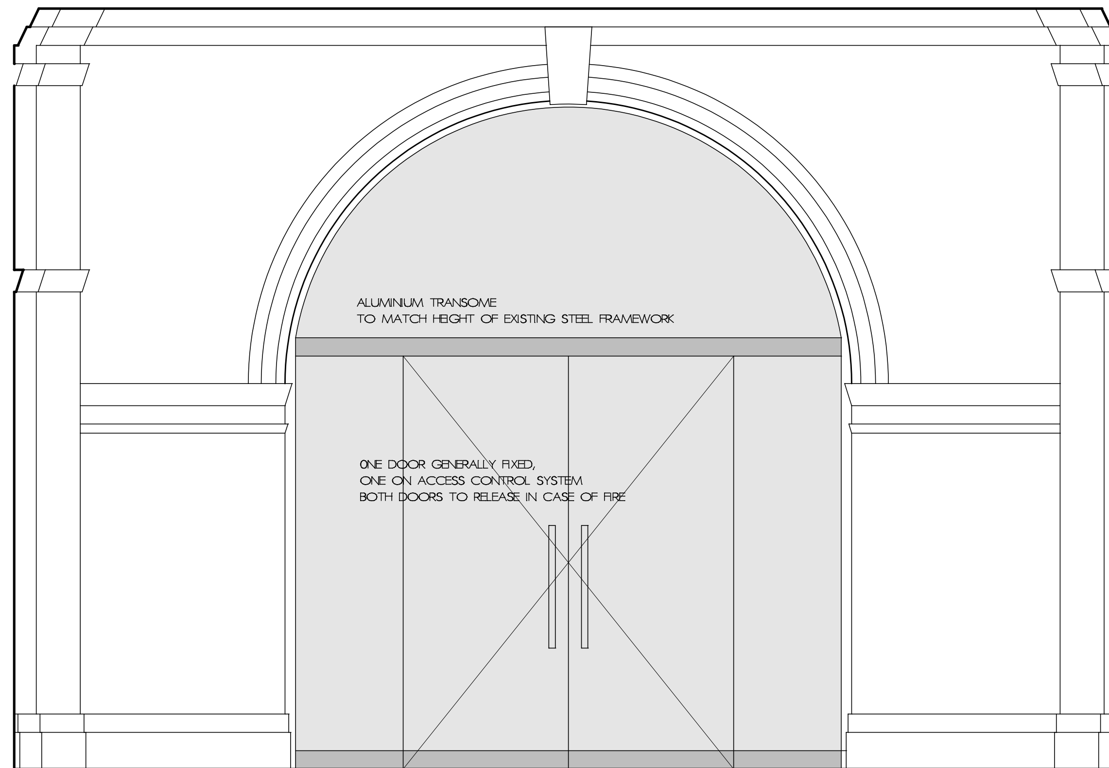
INTERNAL ELEVATION 1:20
