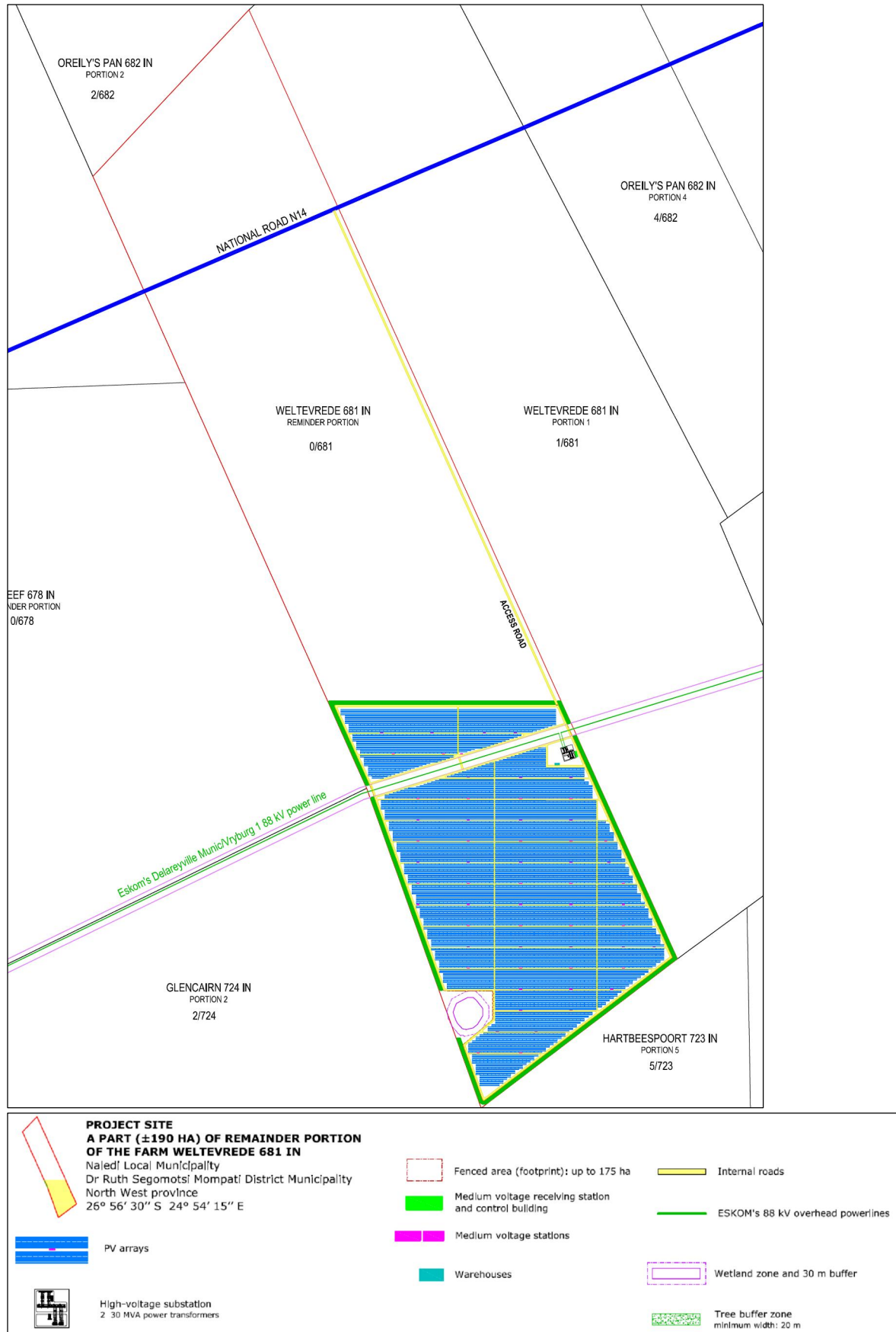
Figure 2 Layout of the Carocraft Solar Park
