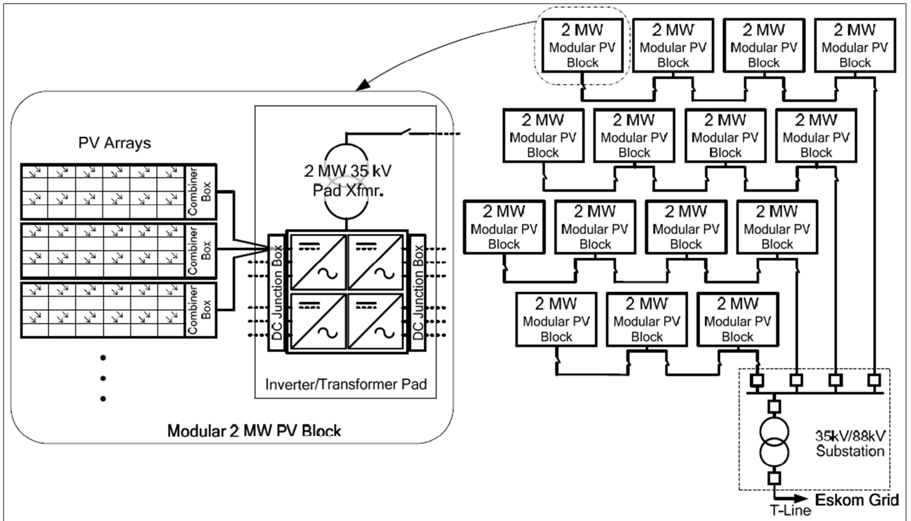
Figure 1: Electrical Conceptual Diagram
