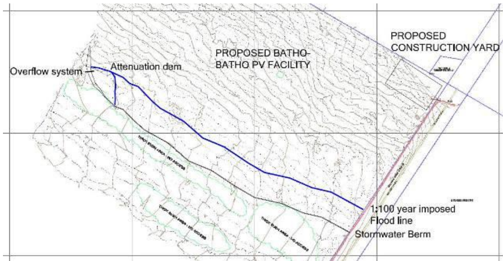
Figure 1: Conceptual Stormwater Plan
