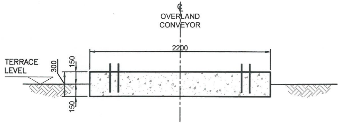
SECTION A SCALE (1:25)
