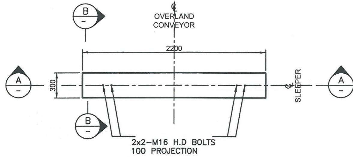
PLAN ON FOUNDATION SCALE (1:25)
