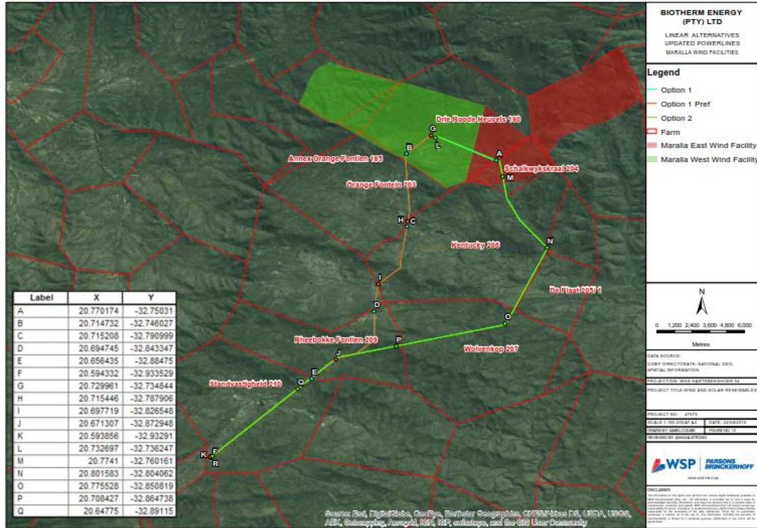
Figure 3-2: Proposed Transmission Integration Line Alternatives
