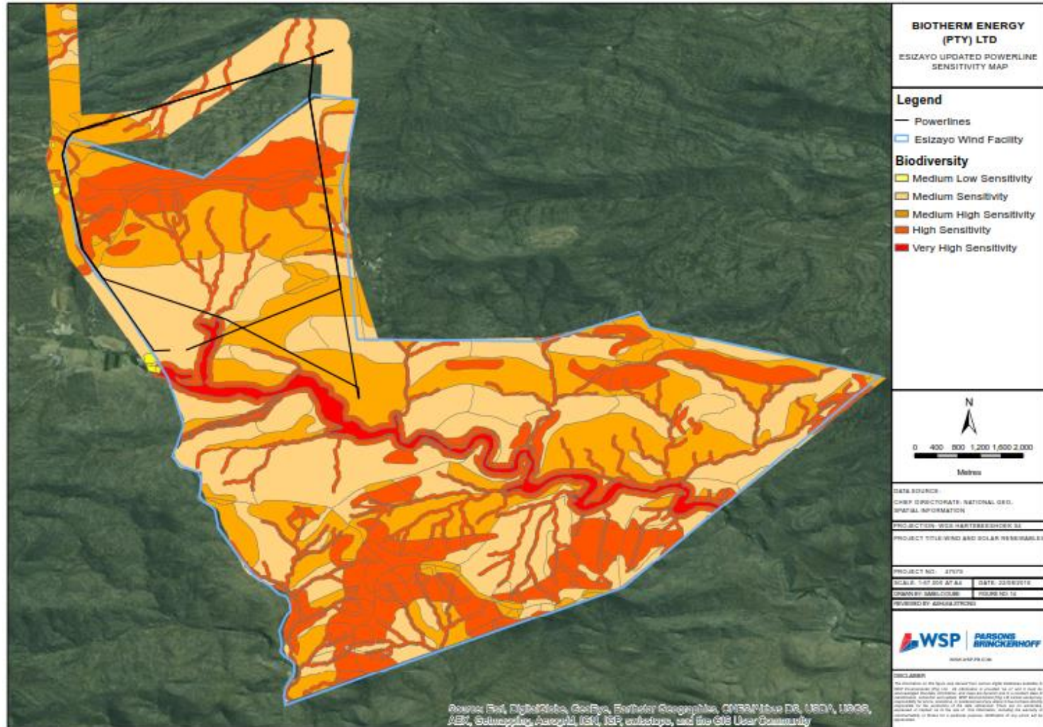
Figure 3-3: Sensitivity Map for the Esizayo WEF Overlain by the proposed layout for the Transmission Integration Project
