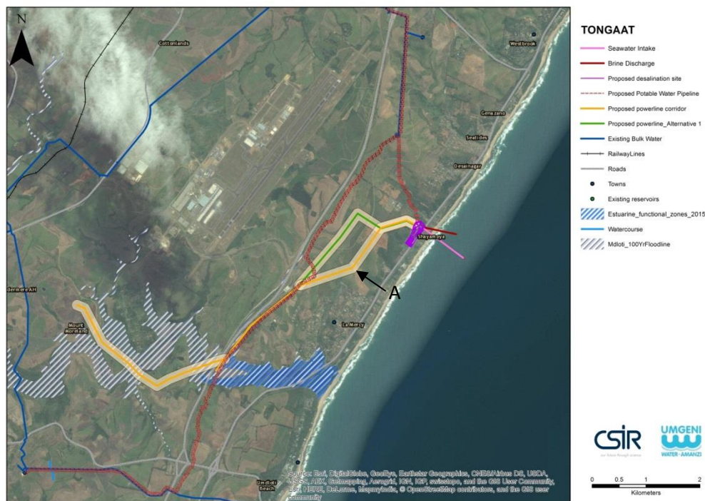
Figure 1: Final layout for the proposed desalination plant and associated infrastructures
