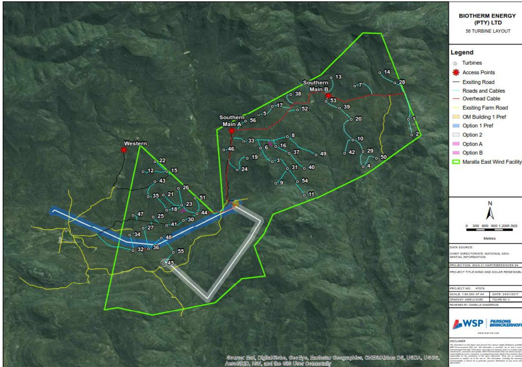
Figure 4 Revised project layout (56 turbines) - Maralla East Facility
