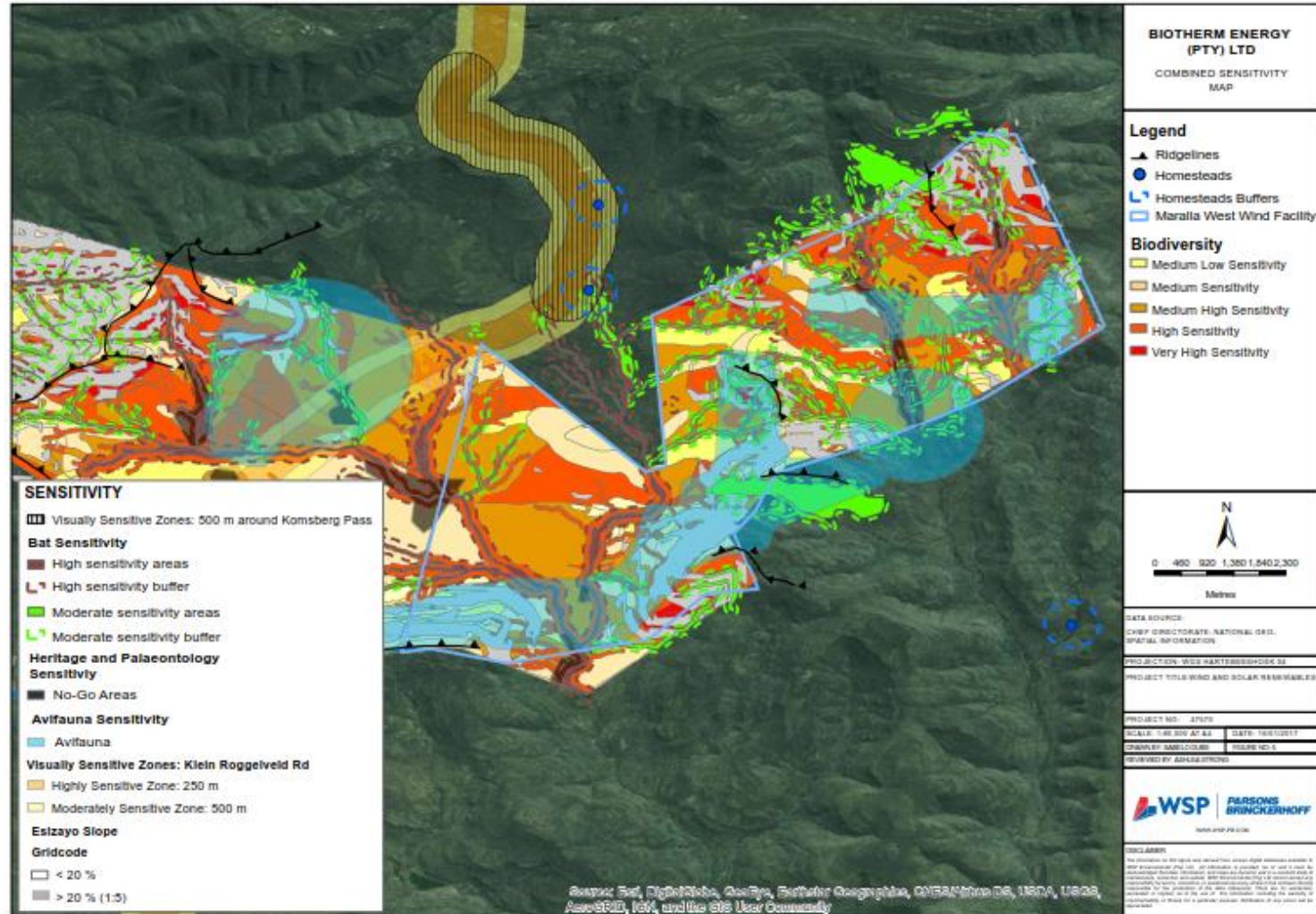
Figure 3-4: Environmental Sensitivity Map for Maralla East WEF
