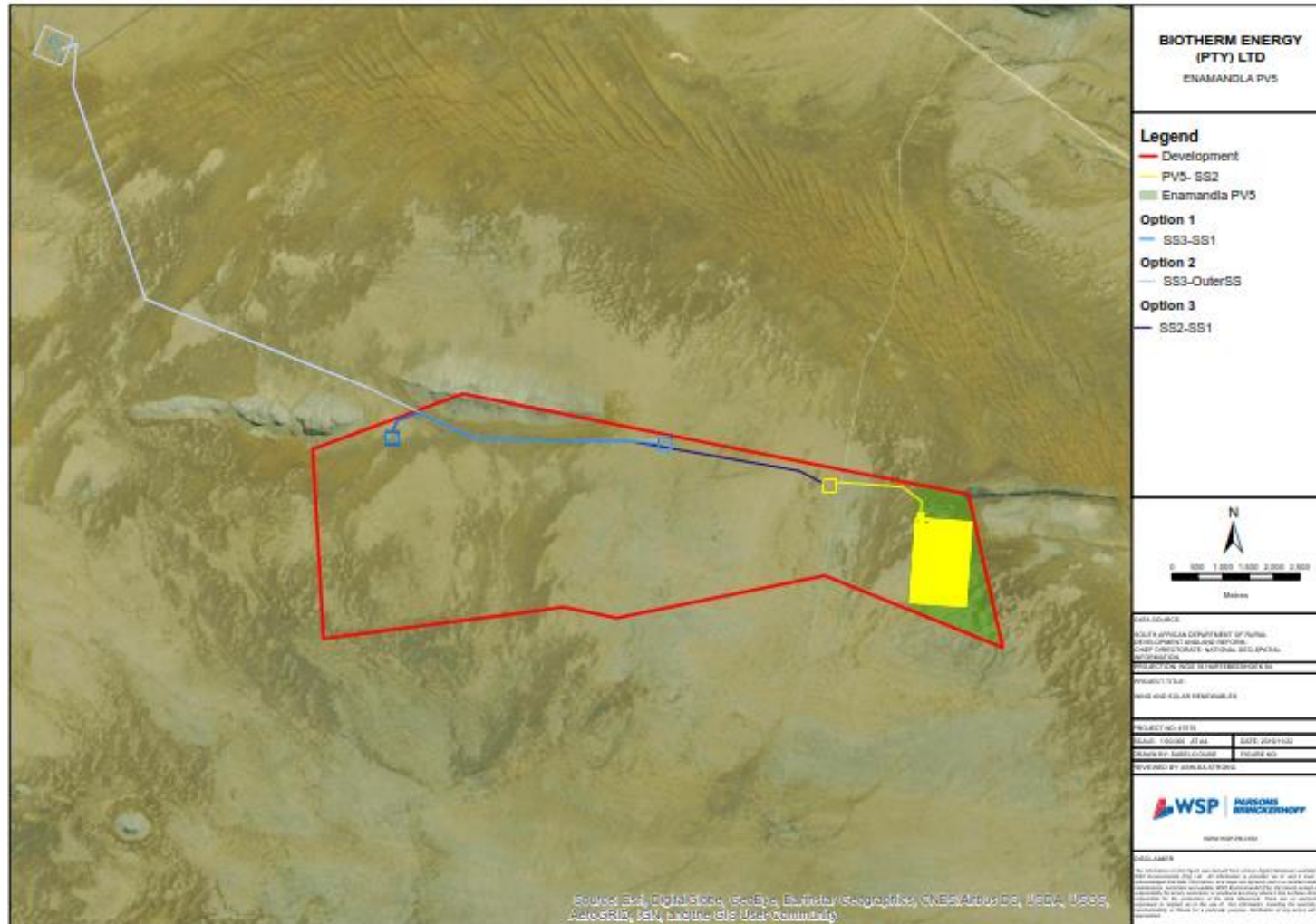
Figure 3-2: Proposed Layout for Enamandla PV 5 (Preferred Alternative)
