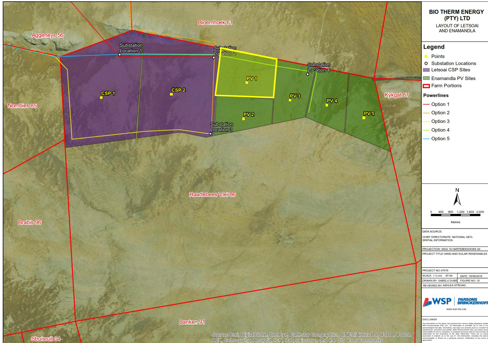
Figure 2 Project layout
