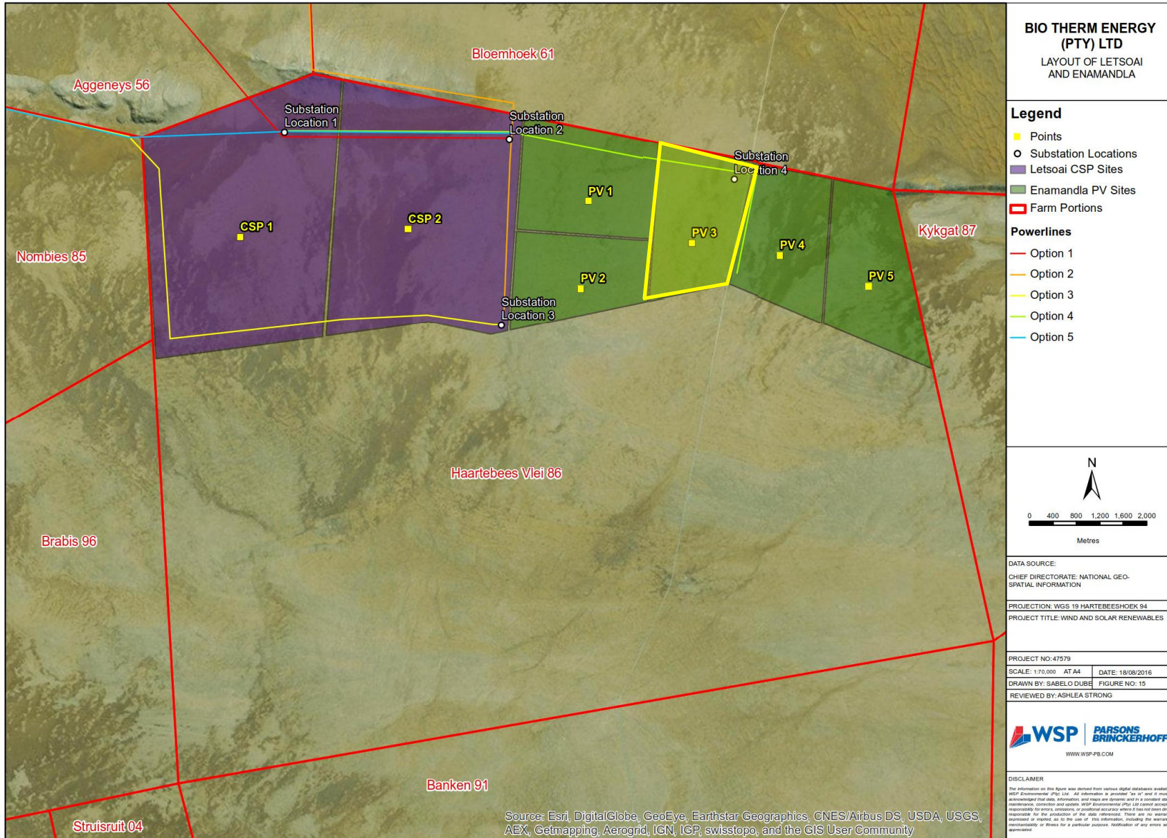
Figure 2 Project layout BioTherm Enamandla Solar Facility - Site 4 BioTherm Energy (Pty) Ltd Public
