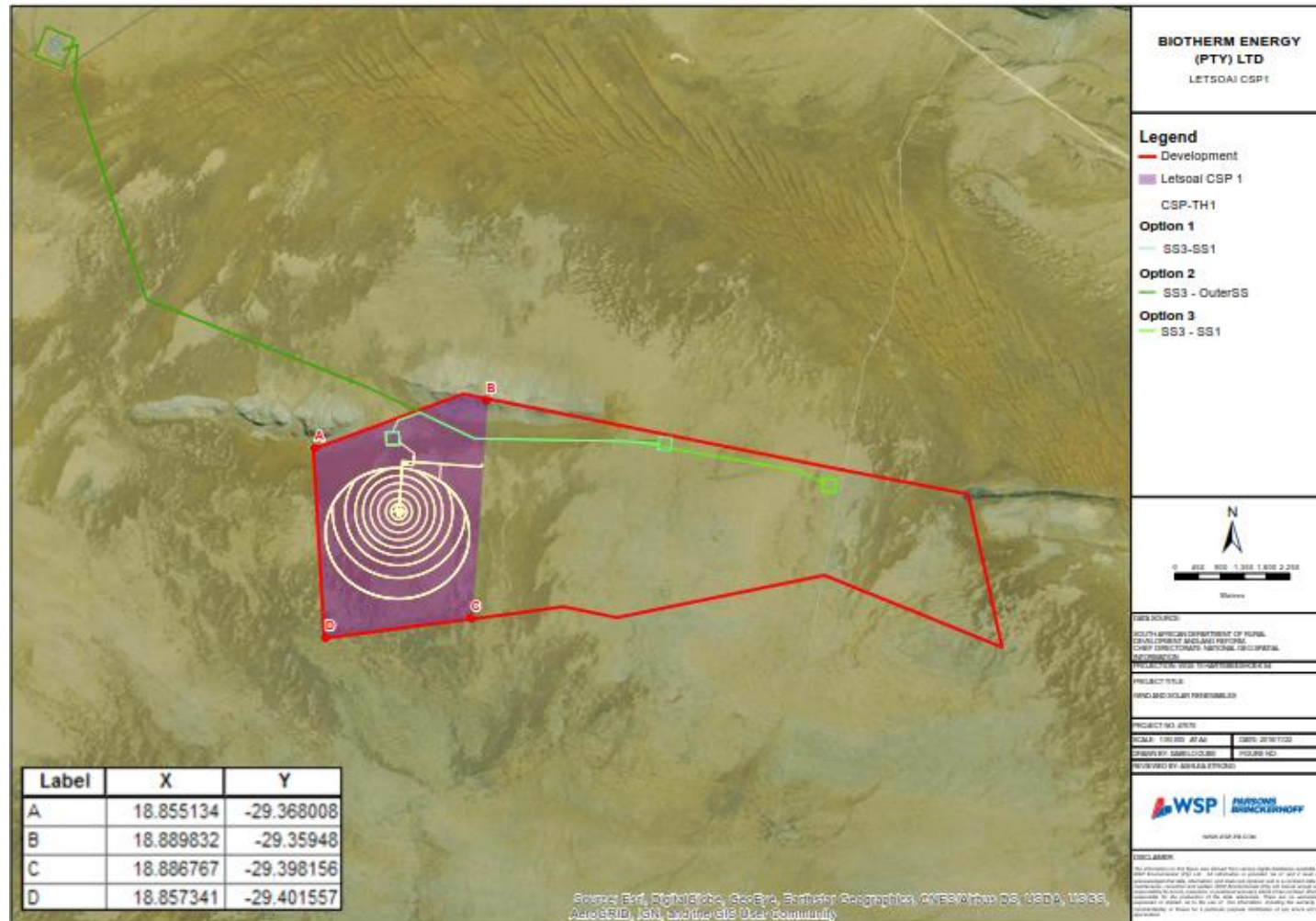
Figure 3-2: Proposed Layout for Letsoai CSP 1
