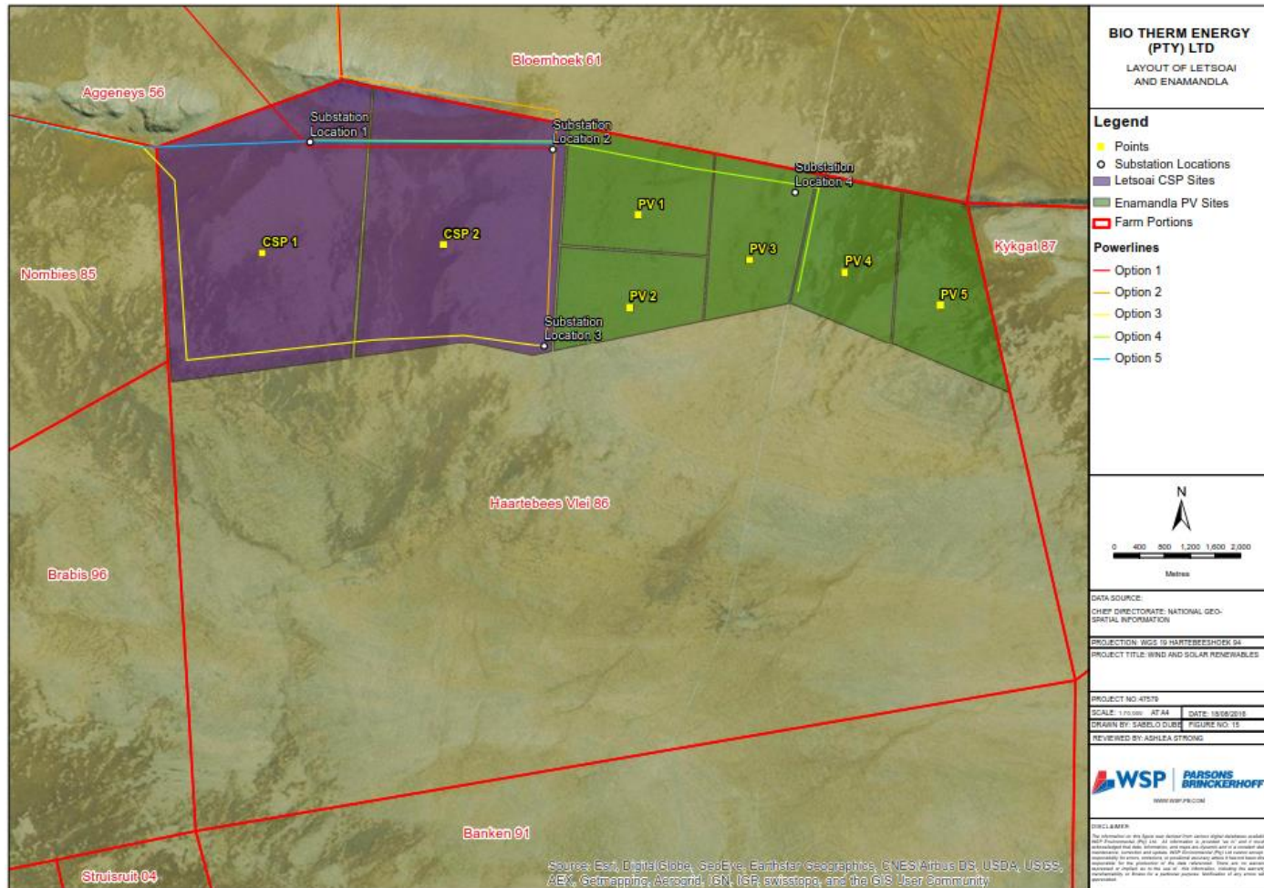
Figure 3-1: Letsoai CSP 1 Location within the Greater Solar Development
