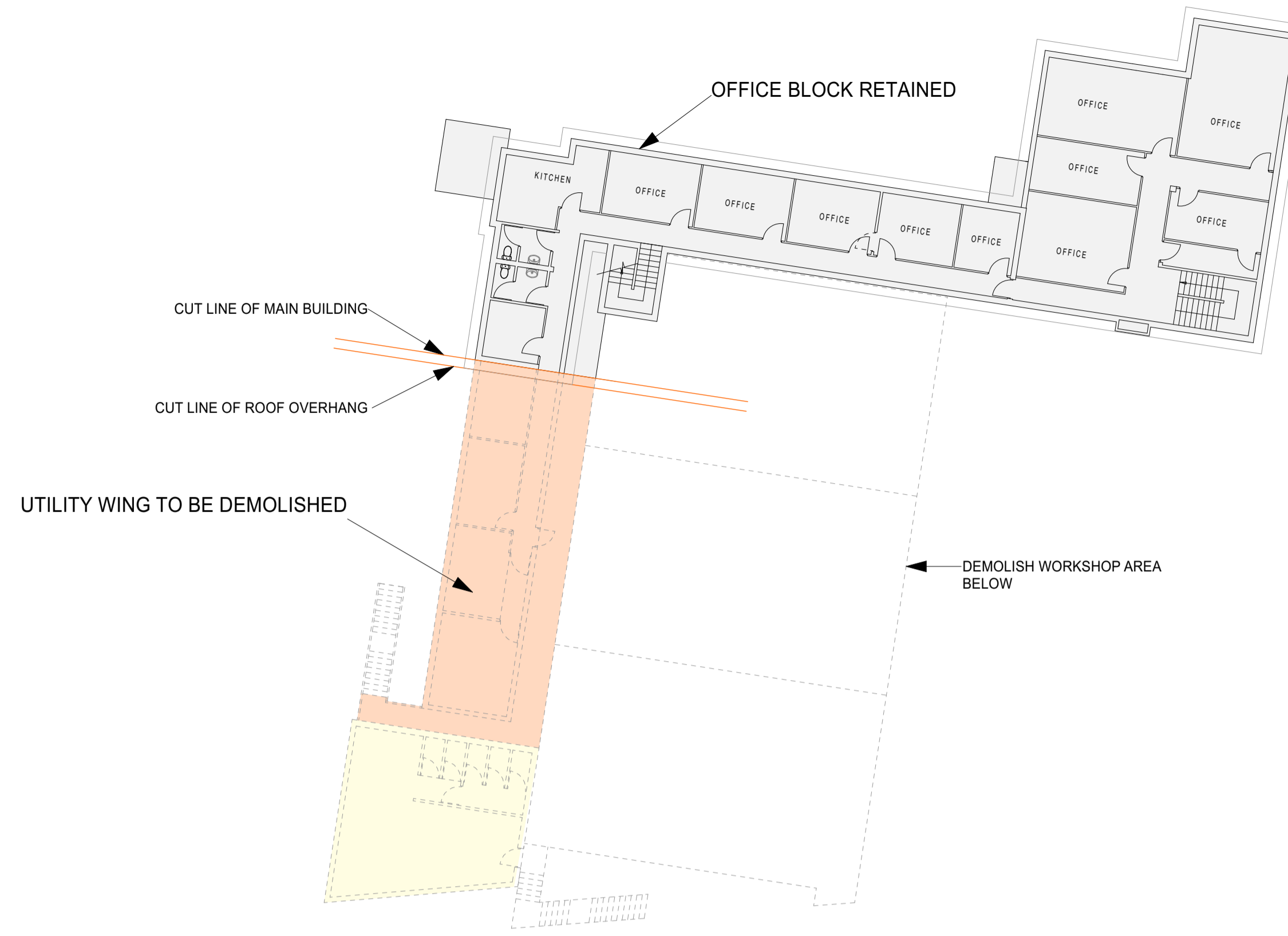
FIRST STORY SCALE 1:200
