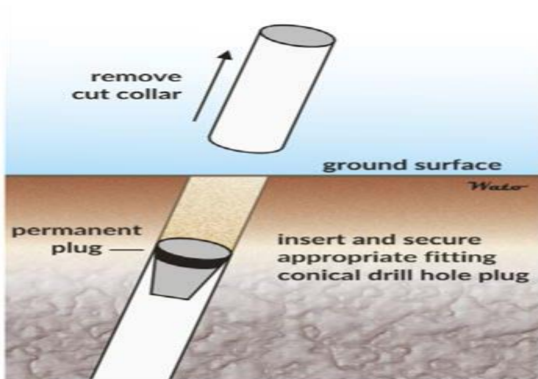
Figure 13: Showing the pvc collar cut at 1 m below the earth surface, the cap is then installed.
