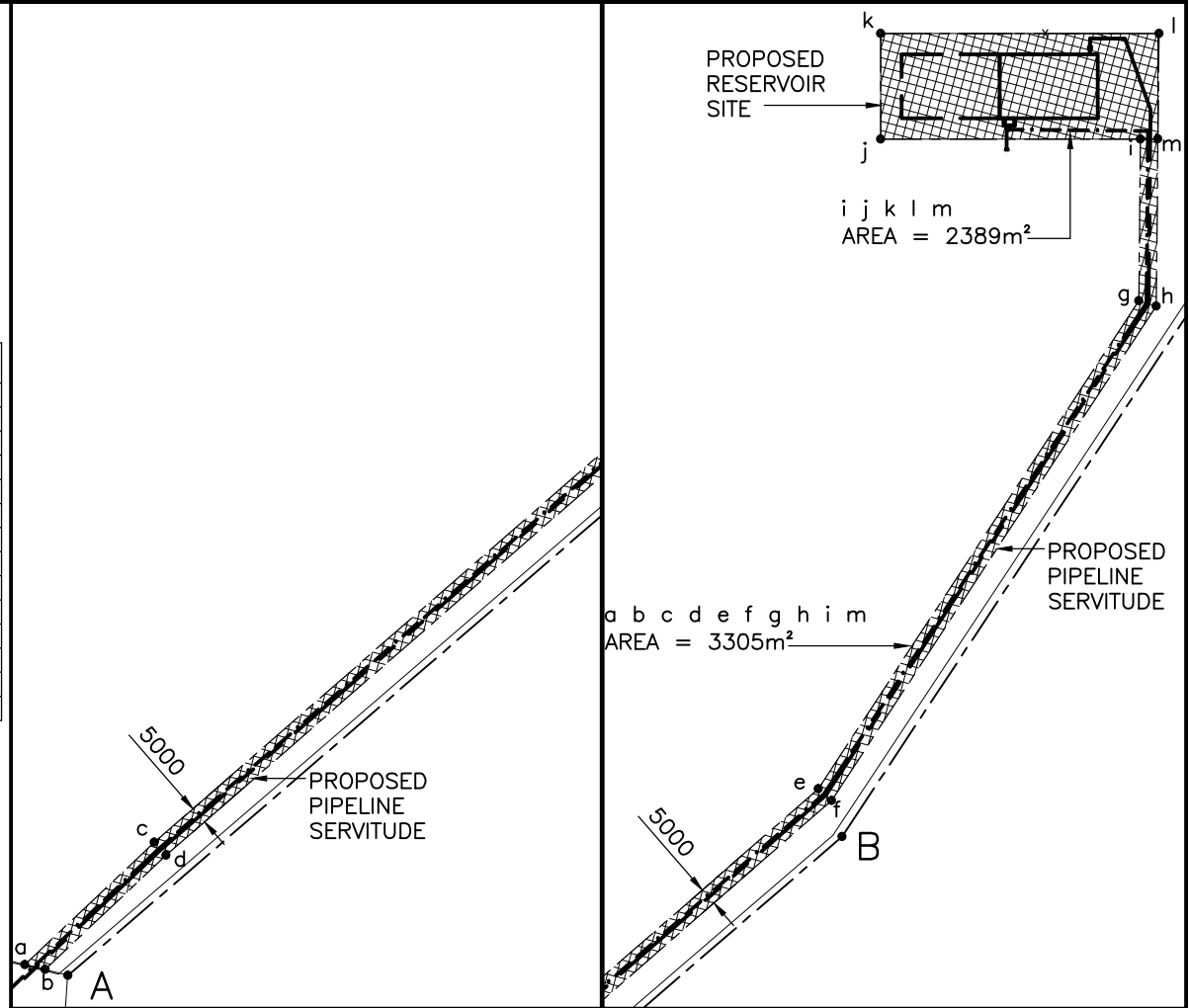
SERVITUDE DIAGRAM NOT TO SCALE
